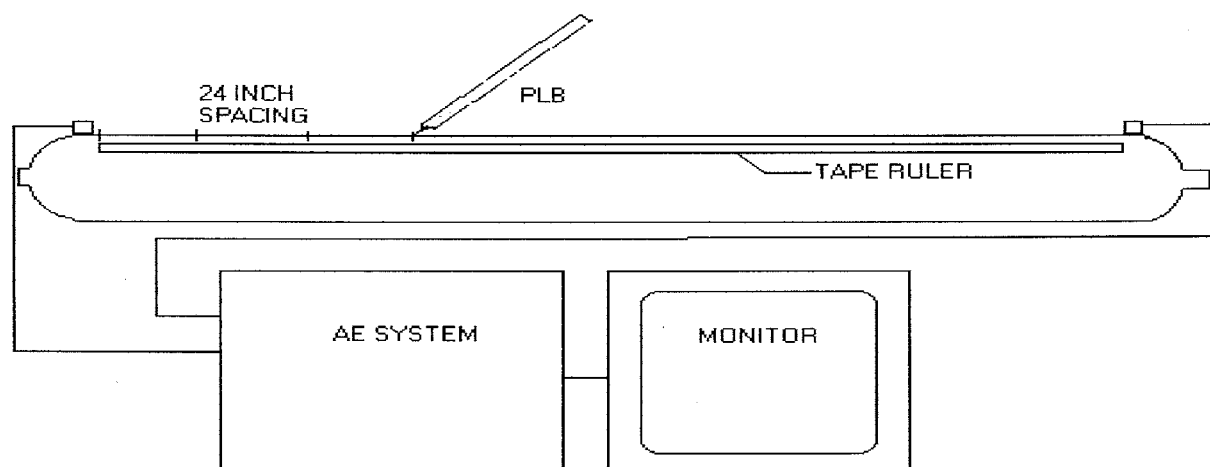
FIG. 2 Illustration of Source Location Performance Verification Process
