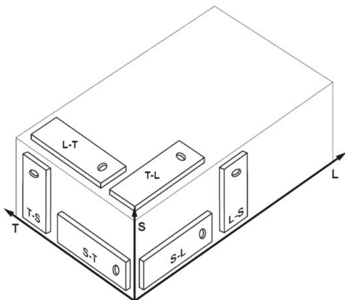
FIG. 5 Grain Orientations and Specimen Orientation Codes for Pin Bearing Specimens Taken from Rectangular Shapes
