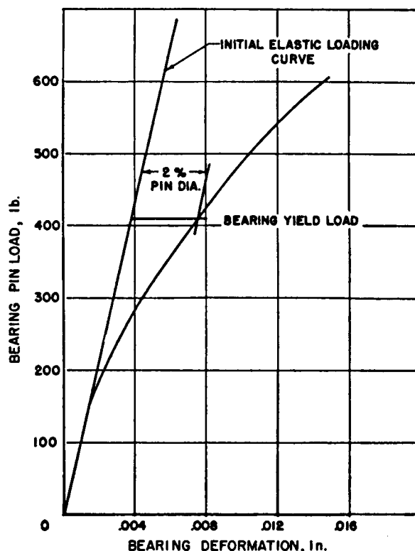
FIG. 6 An Autographic Bearing Load Versus Bearing Deformation Curve on AZ31A-H24 Sheet at Room Temperature
