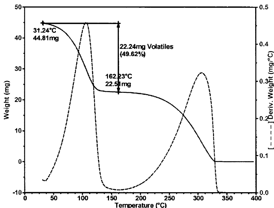
FIG. 1 Determination of Mass Loss for Medium Mass Loss Material
