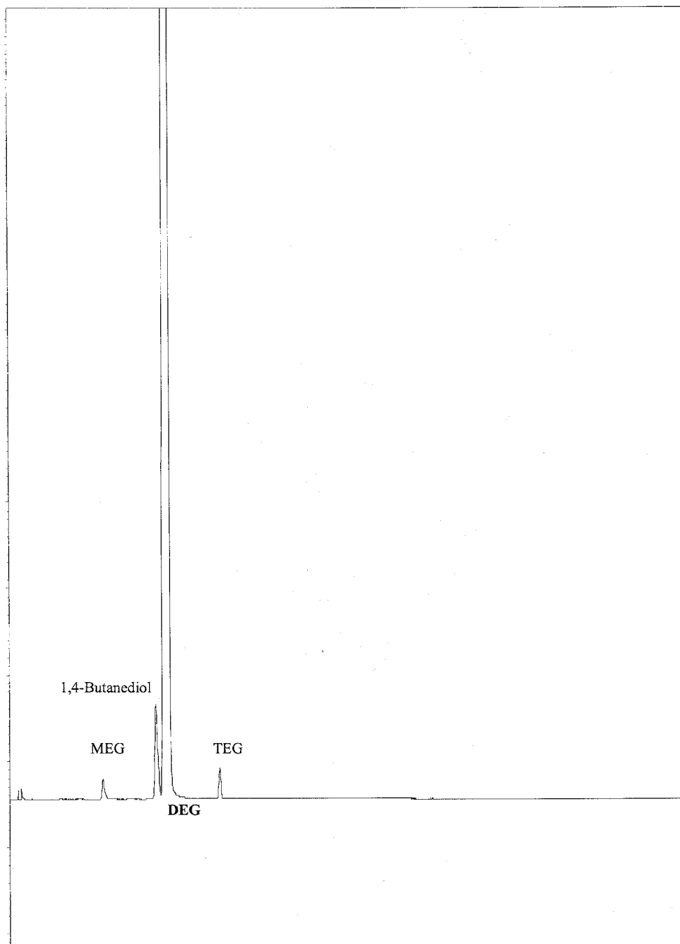
FIG. A1.2 Chromatogram of Impurities in DEG
