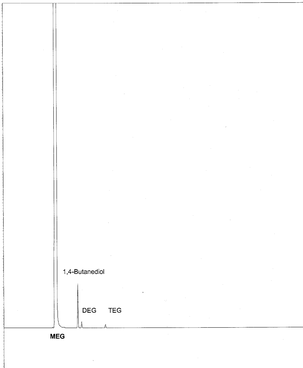
FIG. A1.1 Chromatogram of Impurities in MEG
