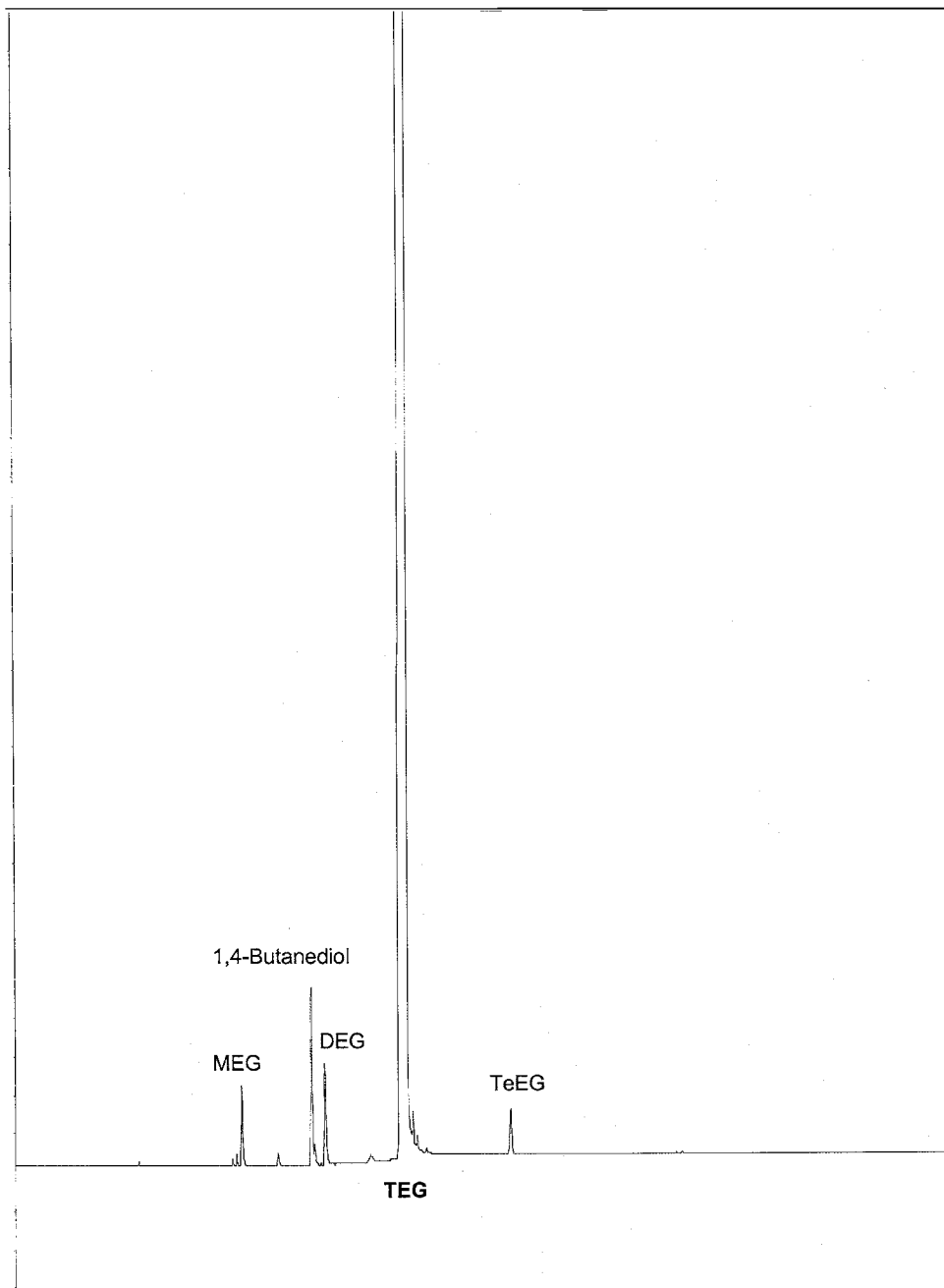
FIG. A1.3 Chromatogram of Impurities in TEG
