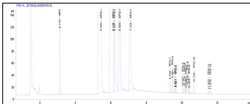
FIG. A1.5 Chromatogram of Glycol Impurities in DPG
