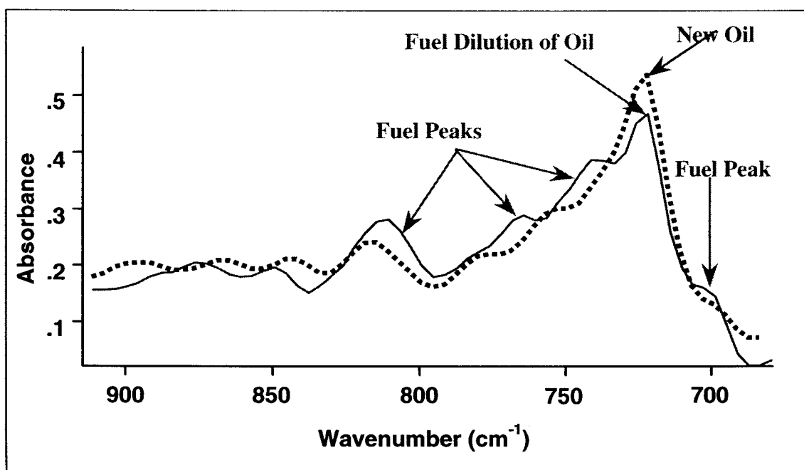
FIG. A1.5 Fuel Measurement in Crankcase Oils
