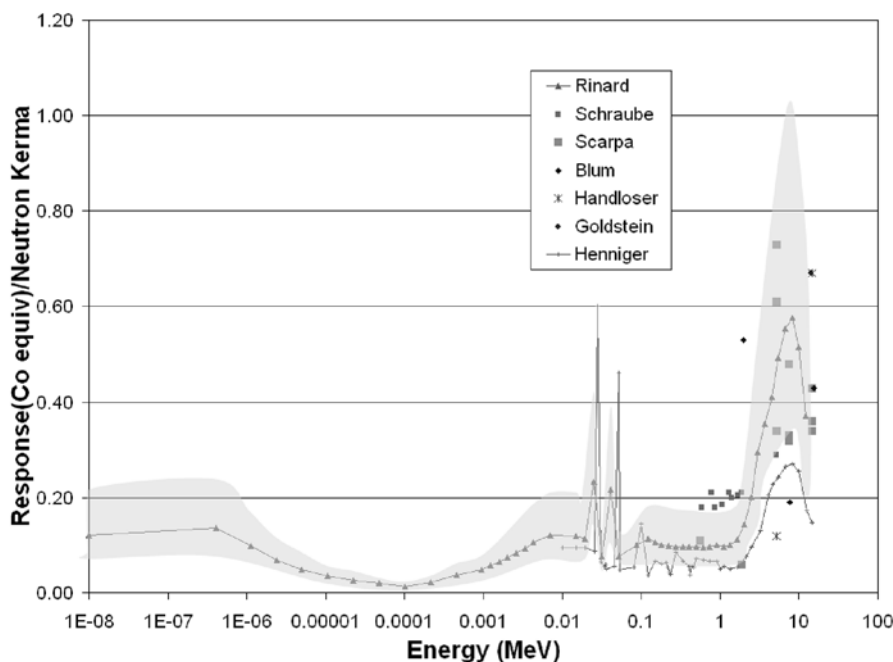
FIG. 2 Relative Neutron Sensitivity of \text{CaF}_2(\text{Mn})
