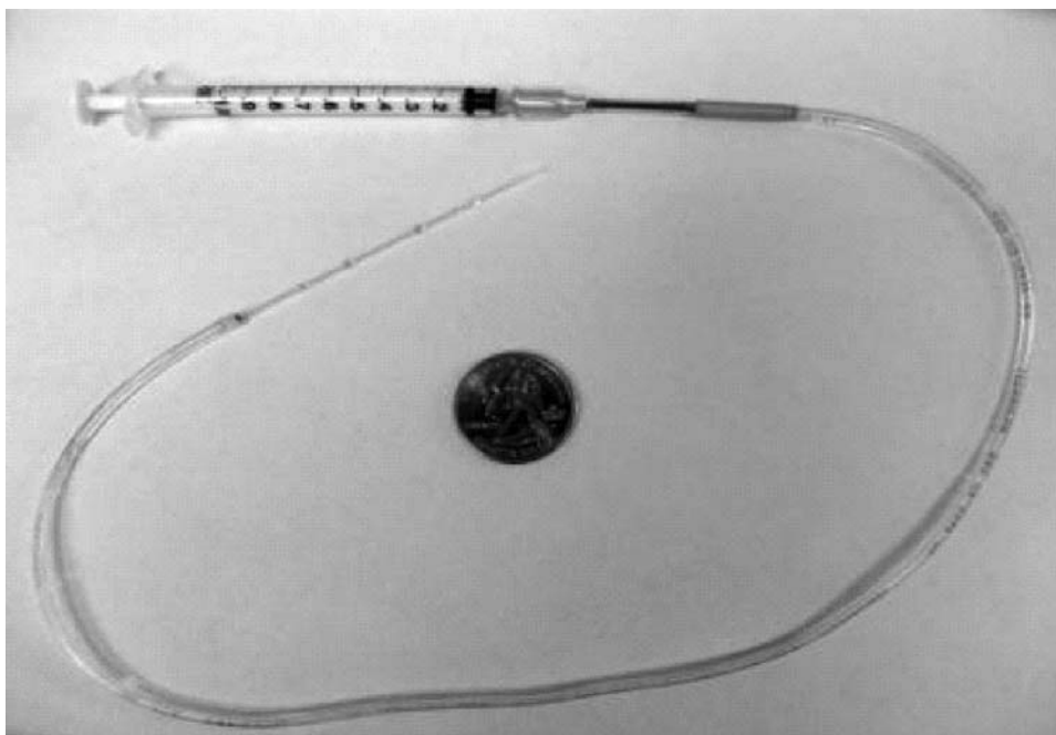
NOTE—The tubing is secured to the needle with a small piece of tape. FIG. A1.1 Syringe Used to Transfer Juvenile Mussels (Wang et al, 2003) (85)
