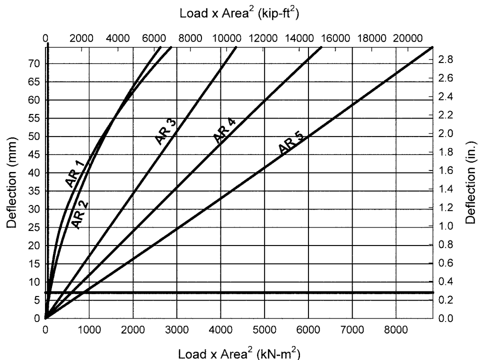
FIG. A3.5 FIG. Deflection Chart for 25 mm (1 in.) Annealed Laminated Glass with Four Sides Simply Supported Showing Lines for Second Design Example
