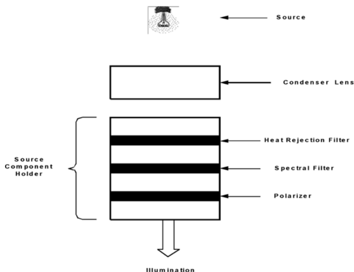
FIG. A1.3 Typical Source Illumination Assembly Unit
