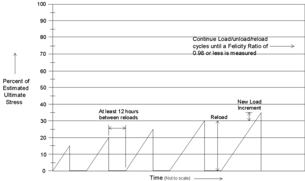
FIG. 2 Loading schedule
