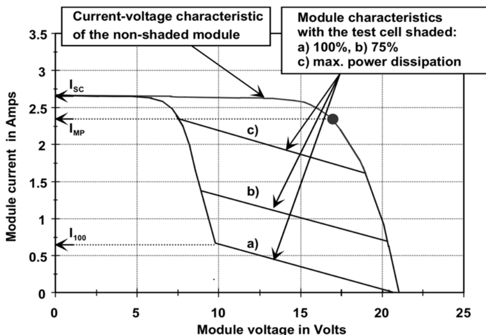
FIG. 4 Module I-V Characteristics with the Test Cell Shadowed at Different Levels
