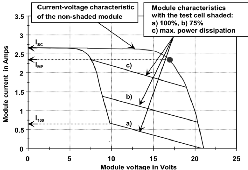
FIG. 4 Module I-V Characteristics with the Test Cell Shadowed at Different Levels
