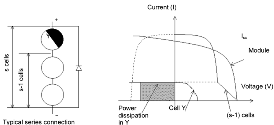
FIG. 2 Bypass Diode Effect
