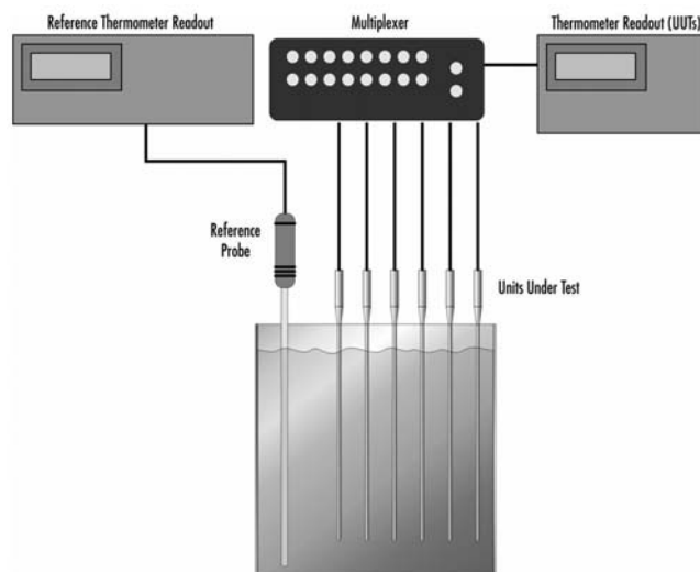
FIG. 4 Block Diagram of Comparison Calibration Setup
