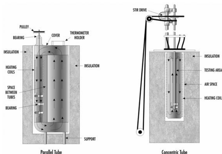
FIG. 1 Alternative Designs of Top Stirred Comparison Baths without Controllers.
