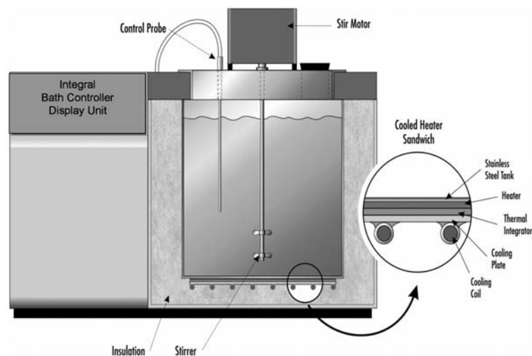
FIG. 3 Sample Design of Comparison Bath with Integral Heating, Cooling and Controller
