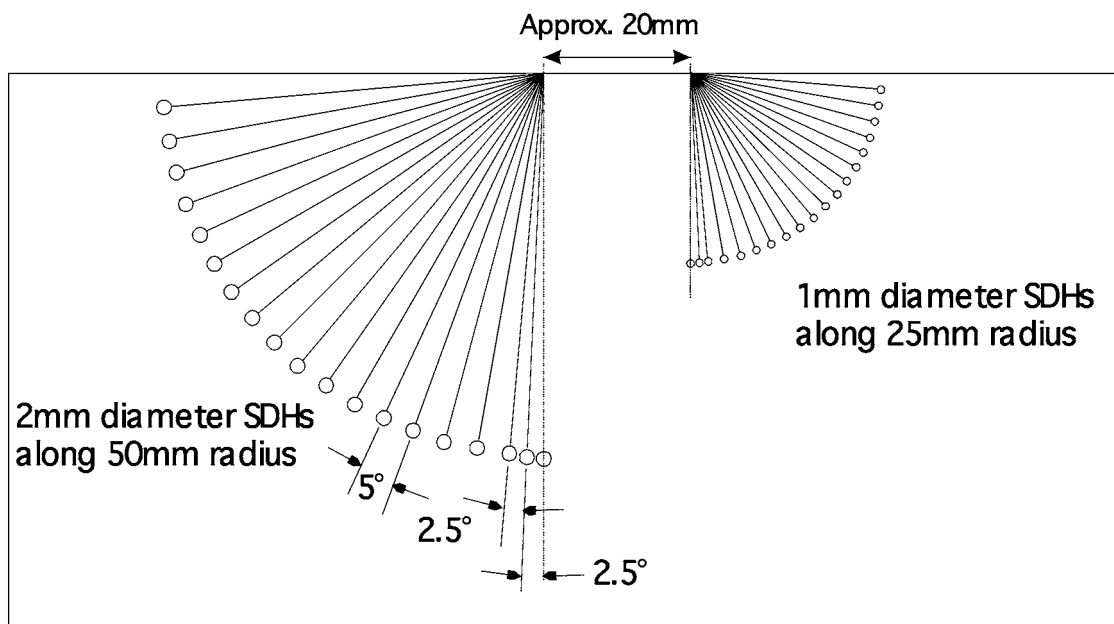
NOTE 1—Block dimensions 150 by 75 by 25 mm (typical) FIG. A2.1 Beam Steering Assessment Block—Constant Sound Path
