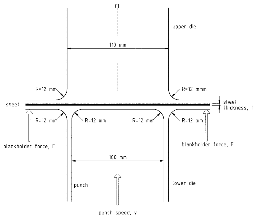
FIG. 1 Cross Section Through the Experimental Setup Used for Cup Drawing
