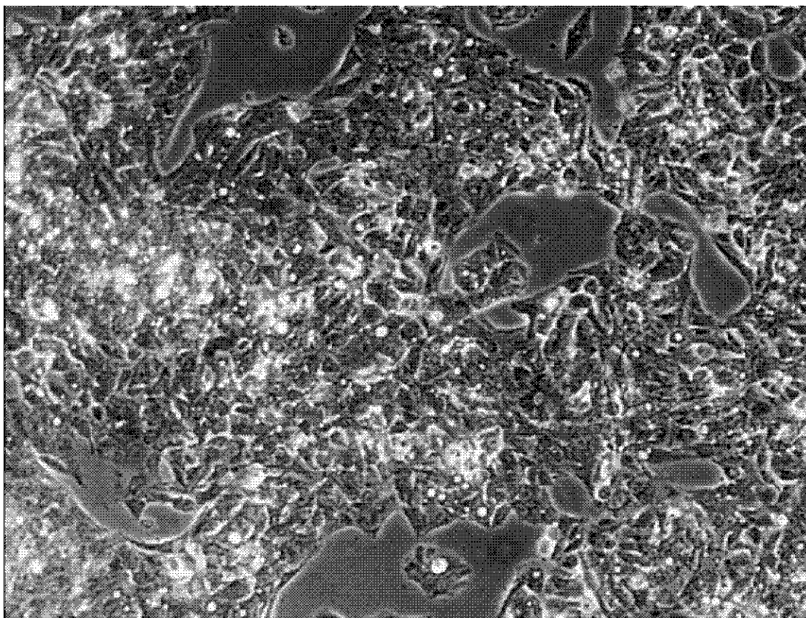
FIG. 2 Example of Hep G2 Cell Culture Appearance
