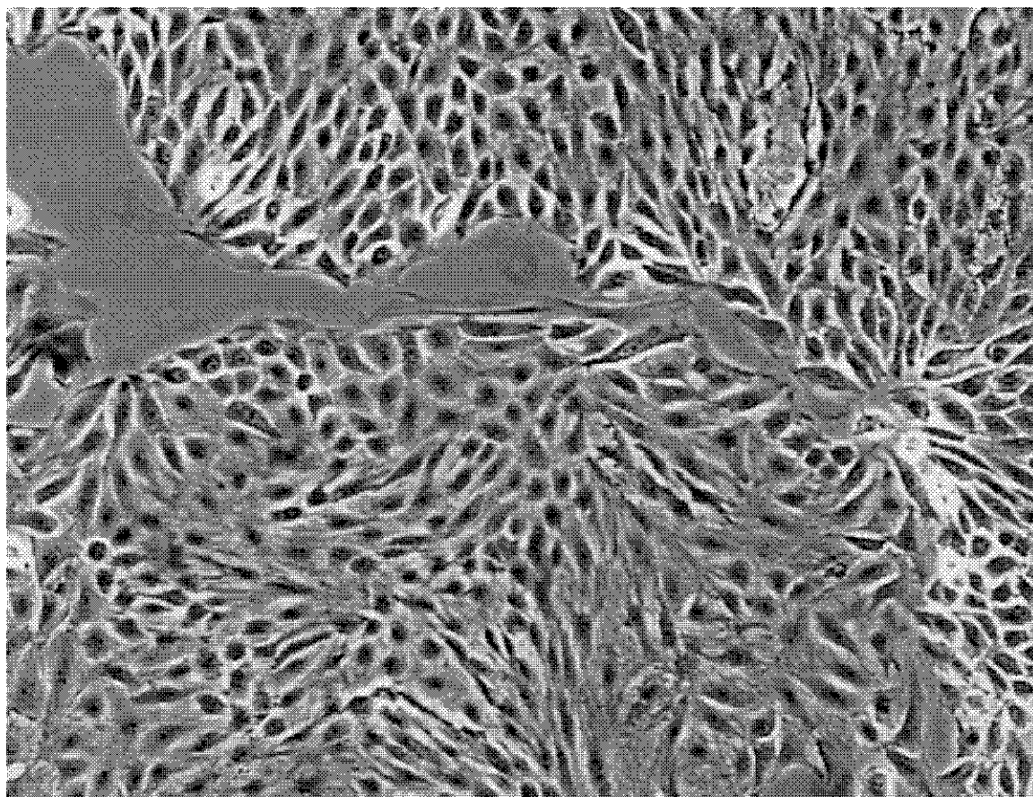
FIG. 1 Example of LLC-PK1 Cell Culture Appearance
