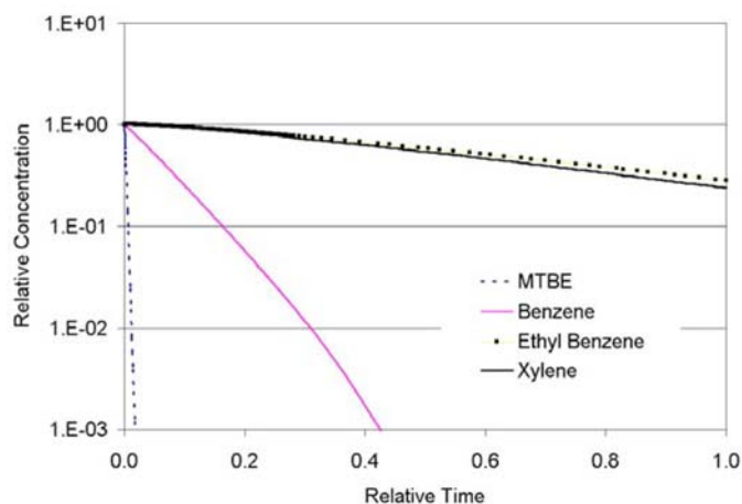
NOTE—In this case, aromatics and MTBE in gasoline are considered. FIG. X3.4 For the Same Hydrogeologic Conditions, the Relative Longevity in the LNAPL Source Varies with Chemical Properties for the Compounds of Interest
