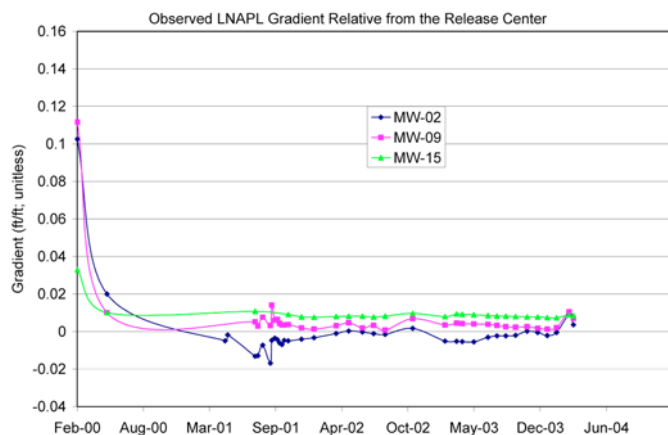
FIG. X6.8 Observed LNAPL Gradient at the Tier 2 Example Site
