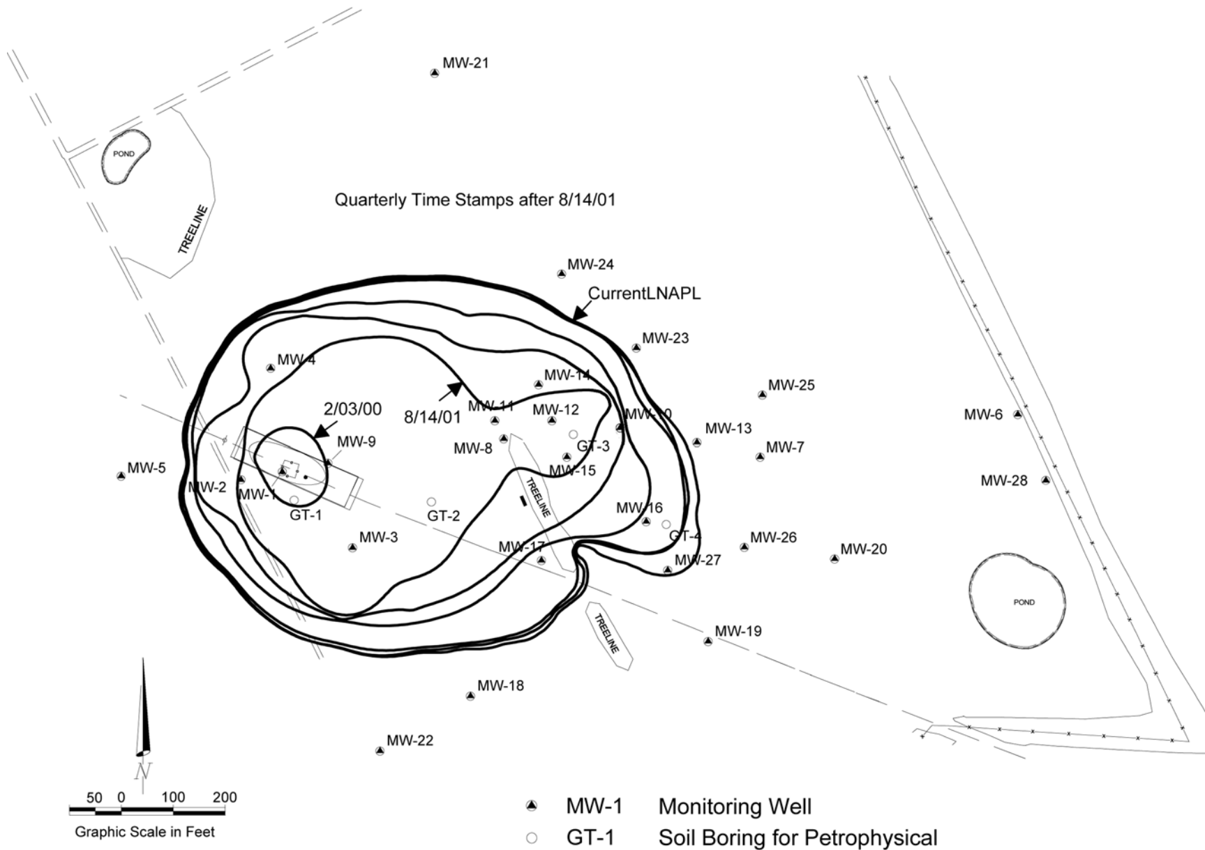
FIG. X6.7 LNAPL Body Through Time
