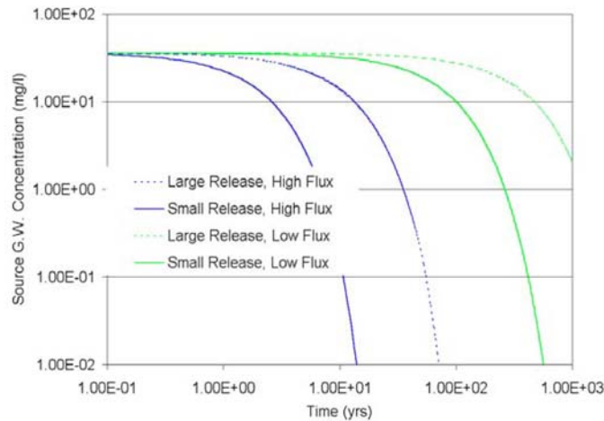
FIG. X3.5 The Potential Longevity of Benzene in the LNAPL Source, Measured as Concentrations in Groundwater, for Large and Small Releases Under High and Low Flux Conditions
