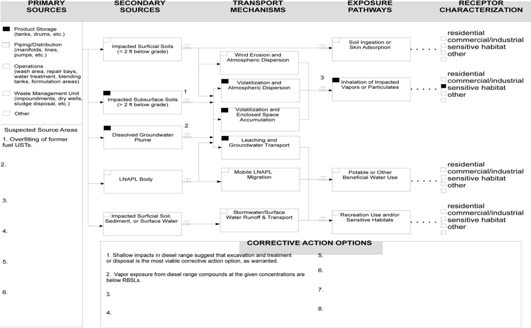
FIG. X6.4 Exposure Pathway Evaluation
