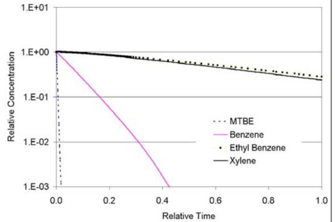
FIG. X3.4 For the Same Hydrogeologic Conditions, the Relative Longevity in the LNAPL Source Varies with Chemical Properties for the Compounds of Interest
