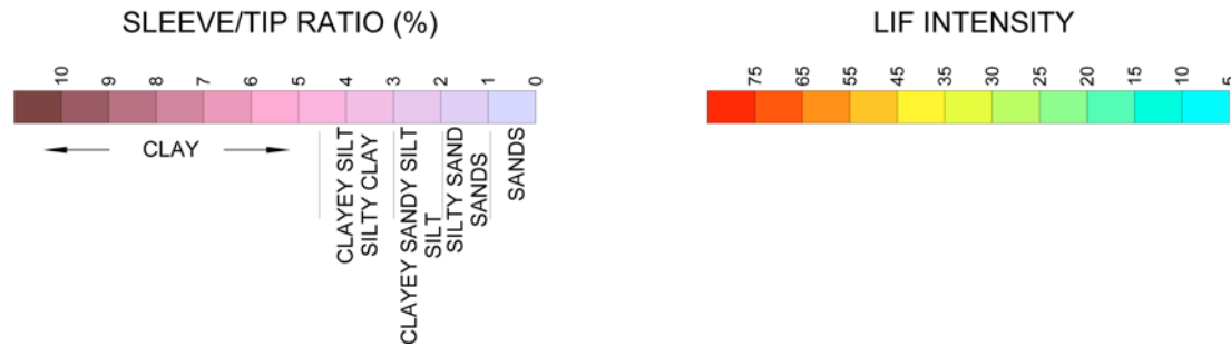
FIG. X6.10 CPT/ROST Cross-Section
