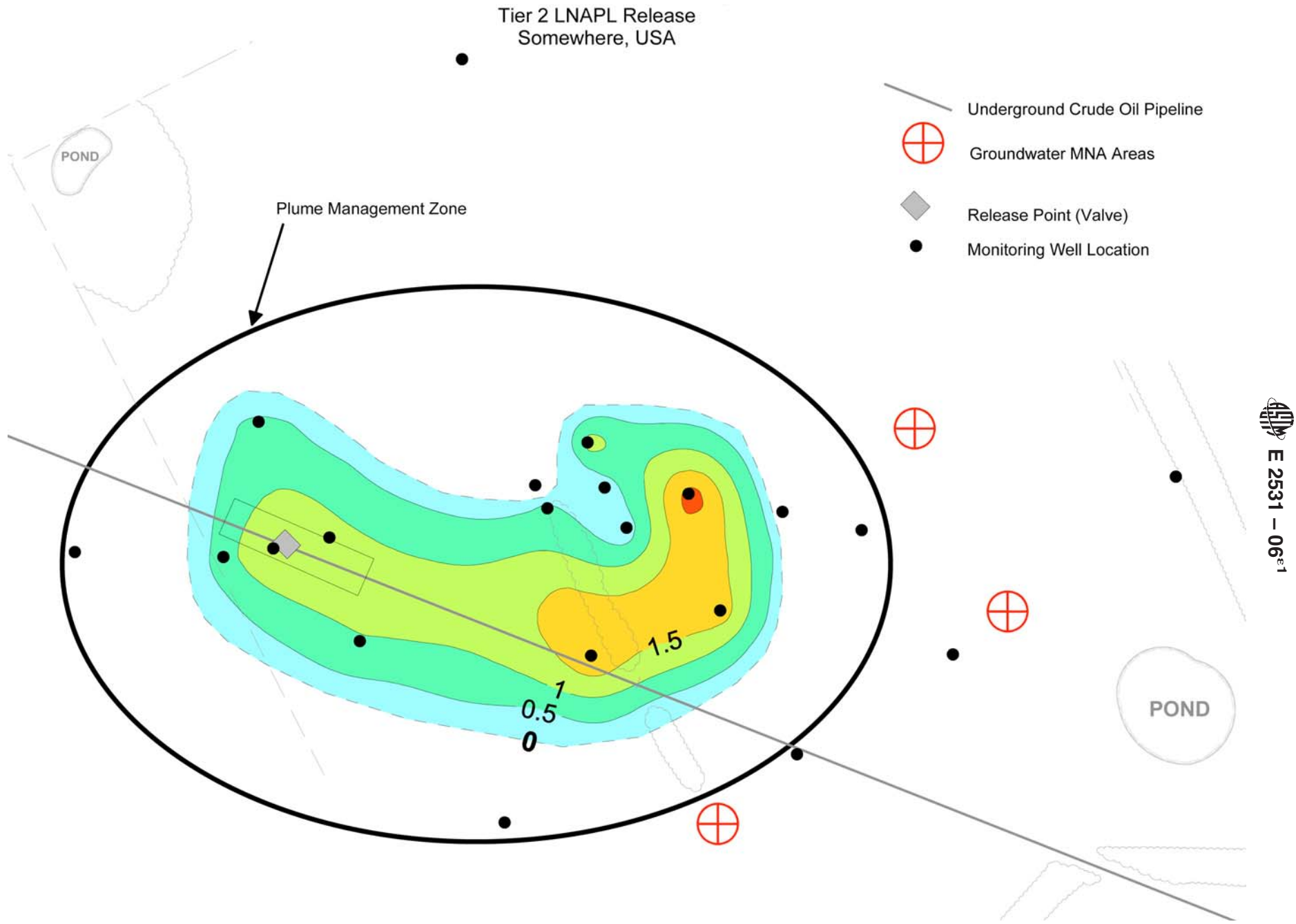
FIG. X6.11 Proposed Solution—Plume Management Zone
