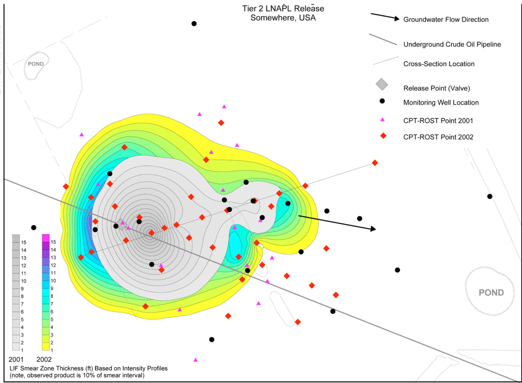
FIG. X6.6 LNAPL Body Through Time
