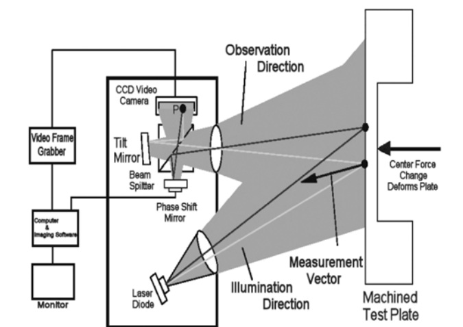
FIG. 3 Schematic Diagram of an Interferometer and Machined Test Plate (Reference Standard) Consisting of a Plate with a Flat-Bottom Hole
