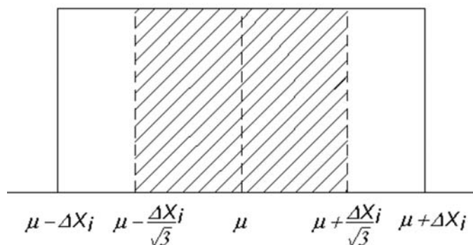
FIG. 1 Rectangular Distribution
