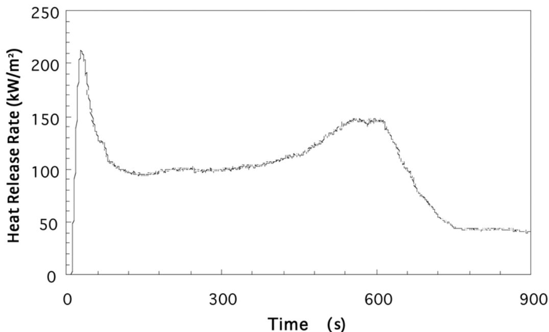
FIG. X1.4 Heat Release Rate versus Time
