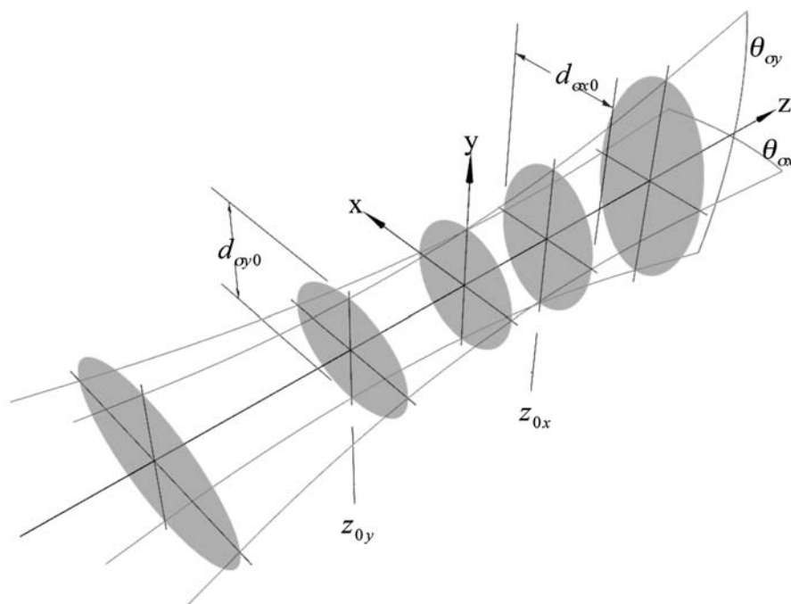
FIG. 1 Schematic Showing Beam Width, Beam Waist, Beam Divergence Angles (Ref ISO 11146)
