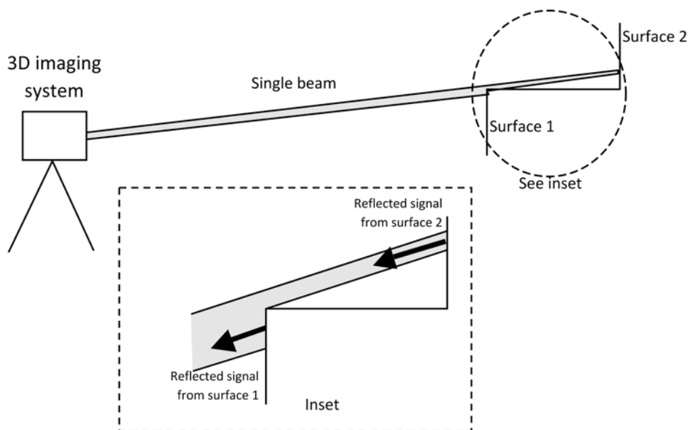
FIG. 6 An Example of Multiple Returns from a Single Object
