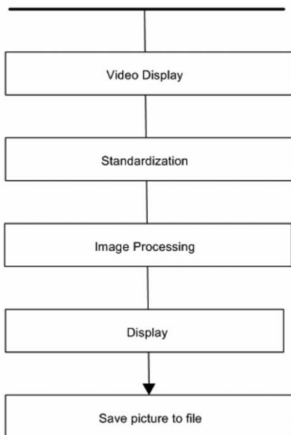
FIG. 5 Typical DSC Application Software Workflow
