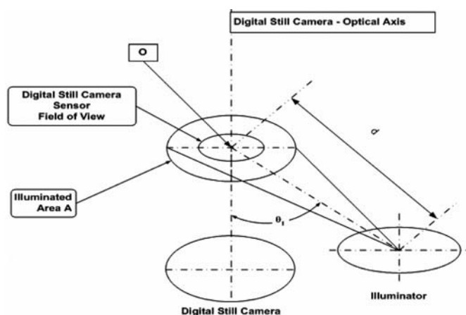
FIG. A1.5 Digital Still Camera System Geometry
