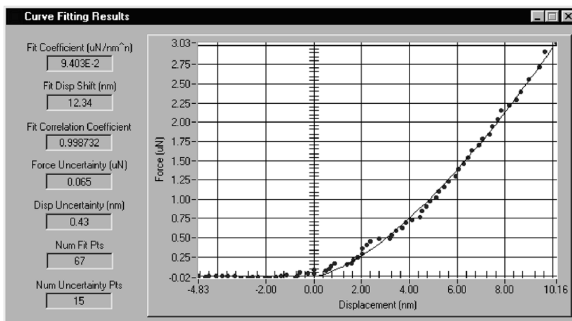
FIG. X1.5 Hertzian Fit to Load-Displacement Curve and Fitting Statistics
