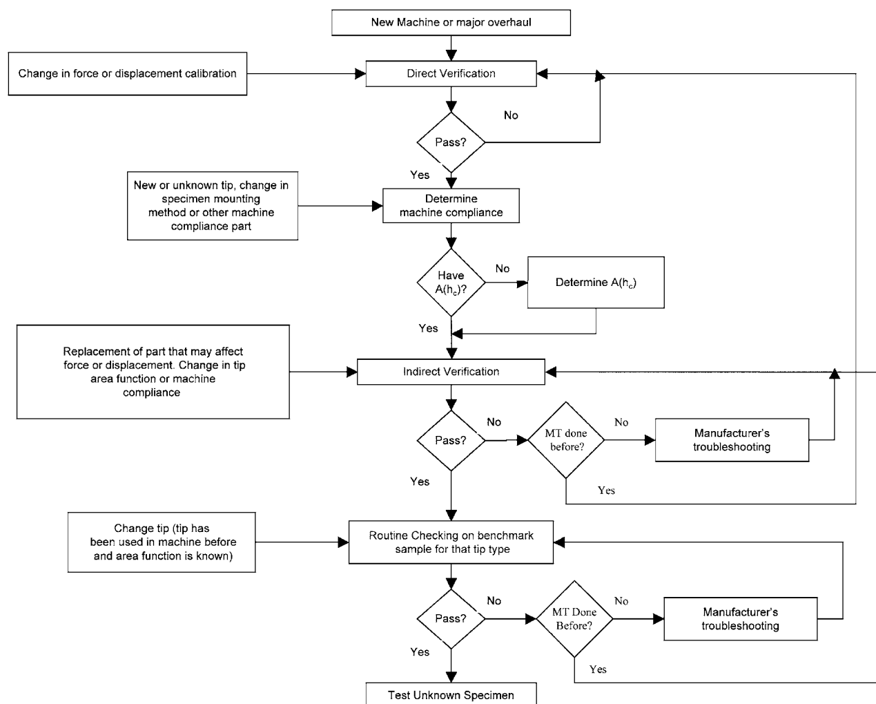
FIG. A1.1 Verification Flowchart
