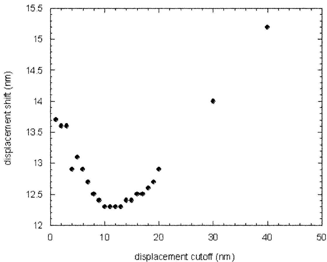
FIG. X1.6 Best-Fit D_s for Various Right-Side Displacement Cutoffs, with Left-Side Displacement Cutoff Fixed at -5 nm
