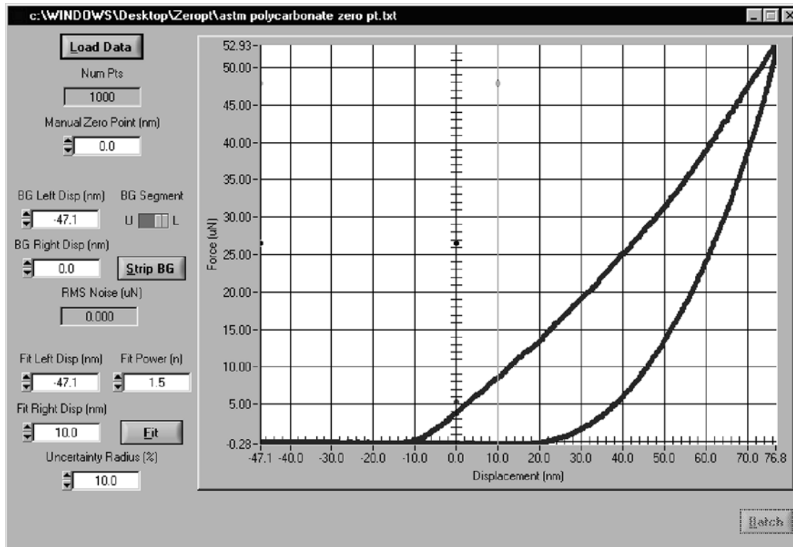
FIG. X1.2 As-acquired Load-Displacement Curve for Polycarbonate
