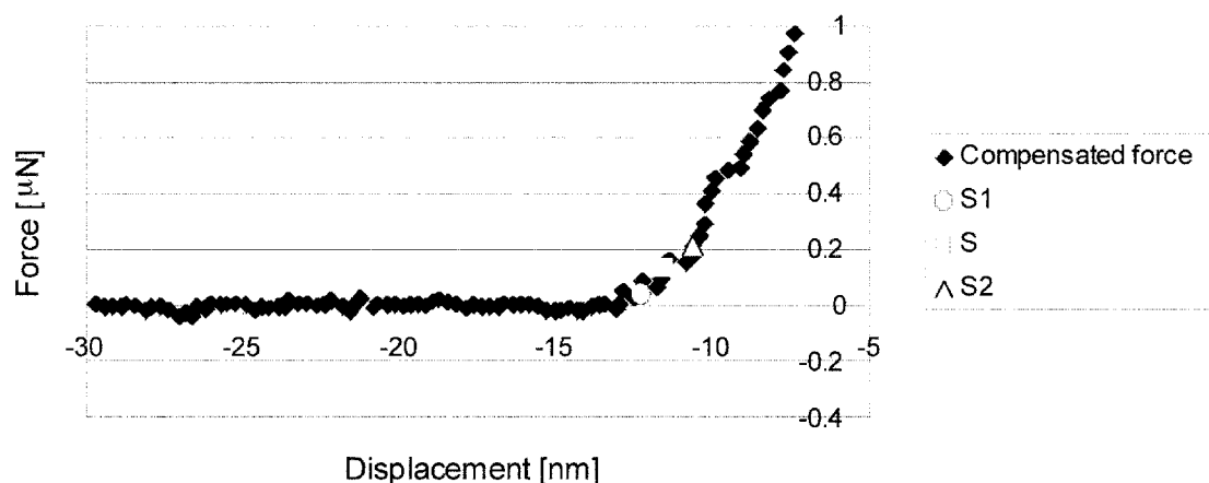
FIG. X1.1 Determination of Zero Point (S) for a Test on Polycarbonate
