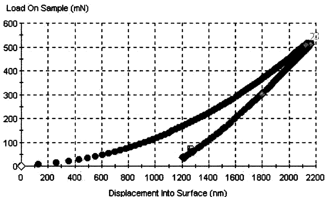
FIG. X4.1 Typical Load versus Displacement ( P versus h ) Curve
