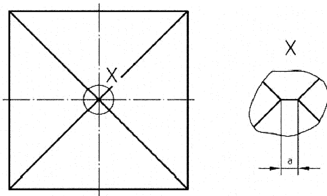
FIG. A3.2 Line of Conjunction at the Tip of the Indenter, Schematically
