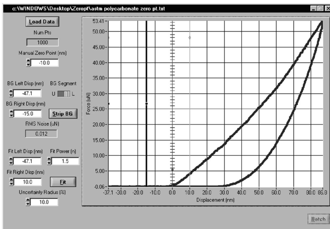
FIG. X1.4 Load-Displacement Curve After Manual Shift of Zero Point
