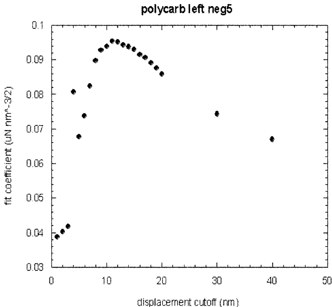
FIG. X1.7 Best-Fit C for Various Right-Side Displacement Cutoffs, with Left-Side Displacement Cutoff Fixed at -5 nm
