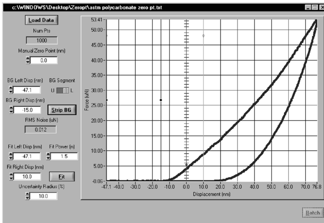
FIG. X1.3 Load-Displacement Curve After Correcting for Residual Slope in Out-of-Contact Load Signal
