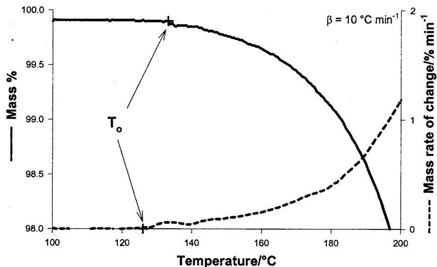
FIG. 2 Zoomed TG and DTG Curves for T_0 Determination
