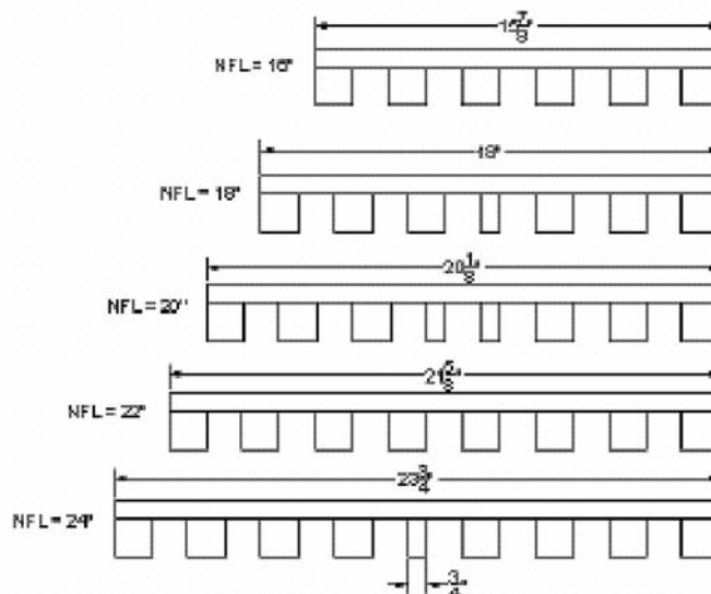
FIG. 9 Kindling Brand 2—Front View For Each NFL
