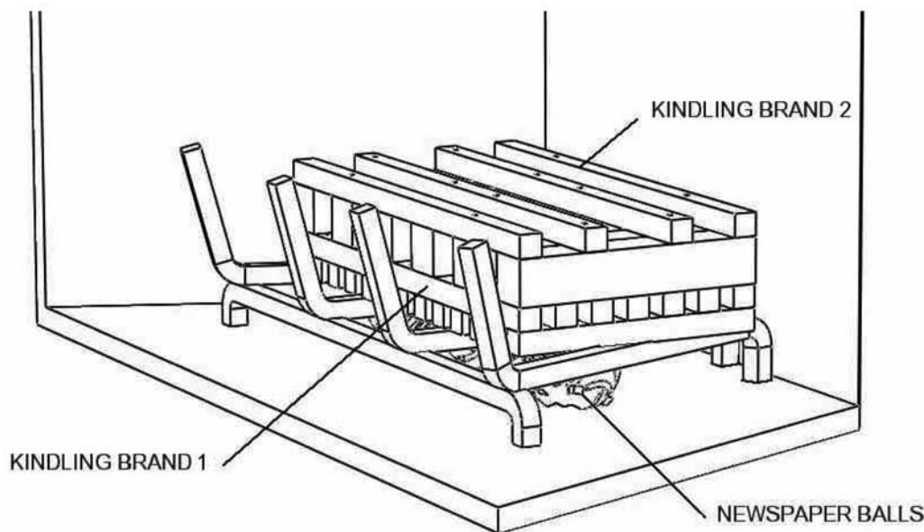
FIG. 13 Newspaper and Kindling (Fireplace with Grate)
