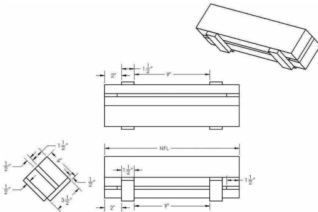
FIG. 12 Third Fuel Crib
