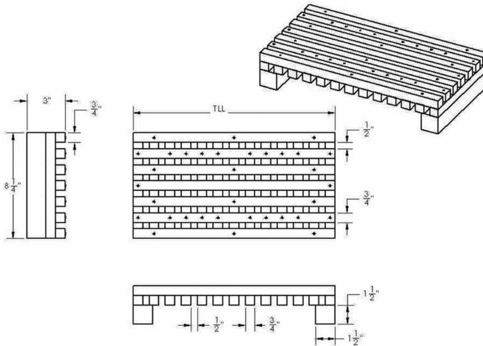
FIG. 5 Kindling Brand 1 (No Grate)
