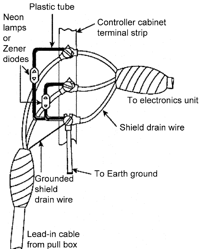
FIG. 6 Lead-In Cable Grounding At The Field Terminal Strip In The Cabinet (9)
