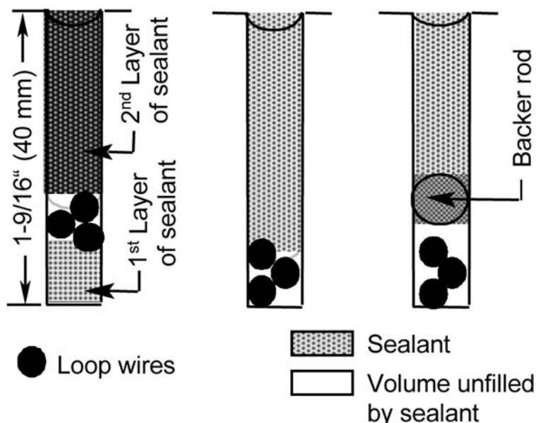
FIG. 4 Sealant Application Methods (9)
