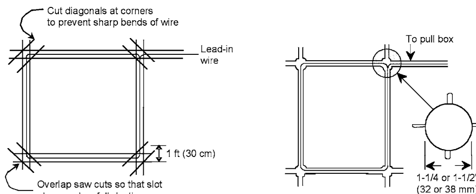
FIG. 2 Saw Cut Corner Treatments (9)
