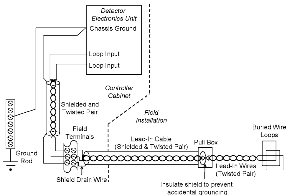
FIG. 5 Inductive Loop Detector System Interconnections (9)
