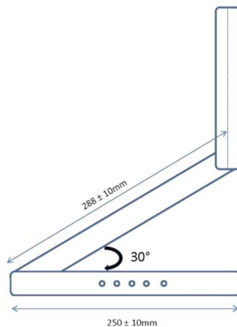
FIG. 3 Side View of Square Gas Burner
