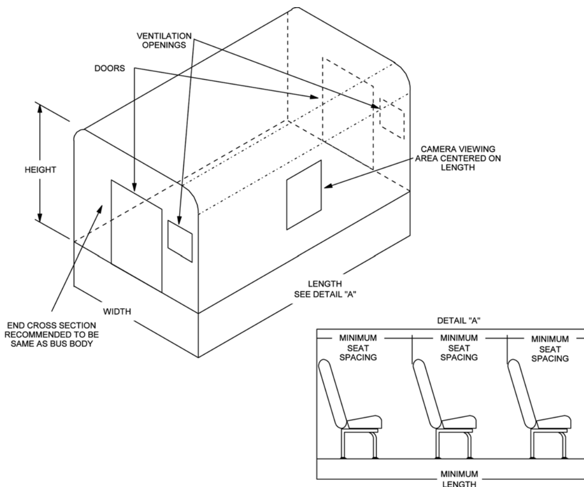
FIG. 1 Test Chamber
