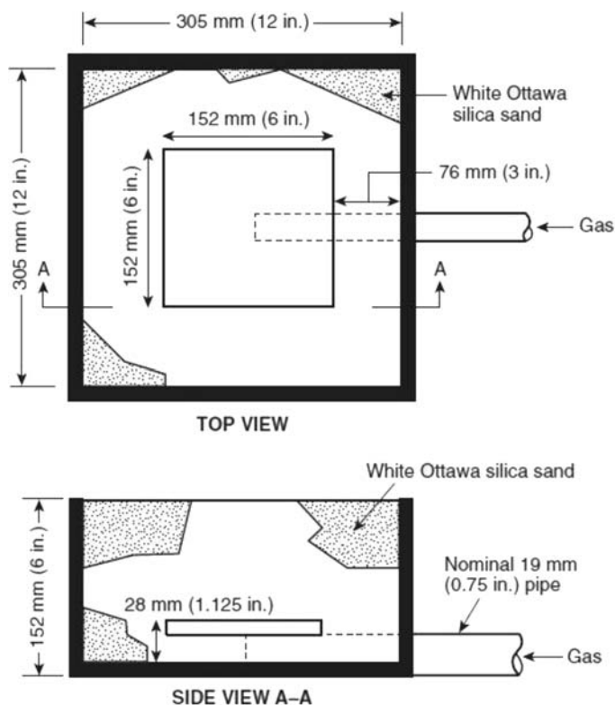
FIG. 8 Ignition Burner for Use Under Seat
