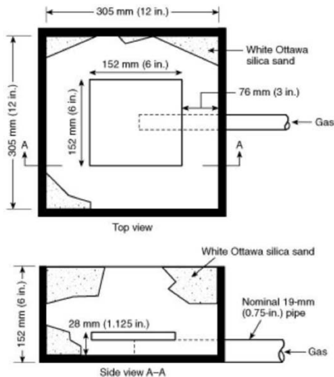
FIG. 5 Ignition Burner for Use Under Seat
