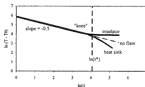
FIG. 1 Logarithmic Temperature-time Plot
