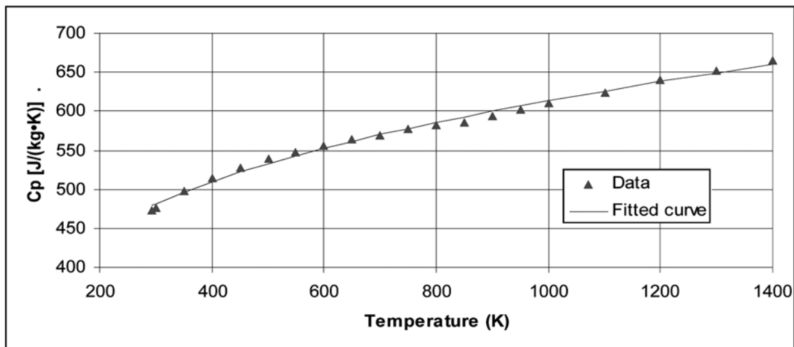
FIG. 3 Literature Values (2) and Fitted Curve for Specific Heat Capacity of 304 Stainless Steel Fitted Curve is of the Form C_p^{SSS} = 6.683 + 0.04906 \cdot T + 80.74 \cdot \ln(T) with T in K
