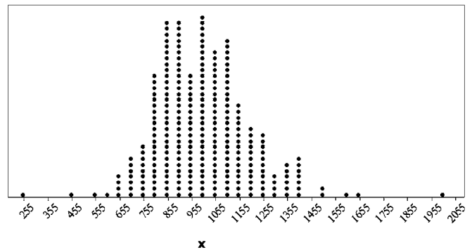
FIG. 8 Dot Plot for Table 11 Data
