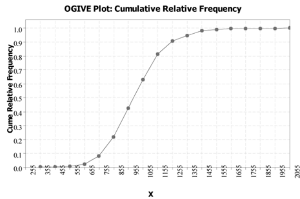
FIG. 10 Relative Frequency Ogive Constructed from Table 12 Information
