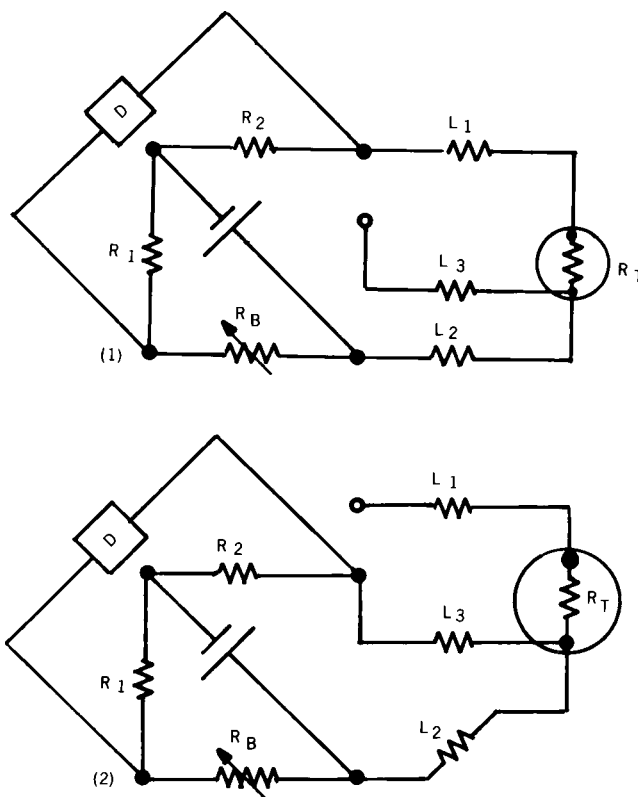
FIG. X1.3 Two Measurement Method for Determining the Resistance of a Three-Wire Thermometer Employing a Simple Bridge
