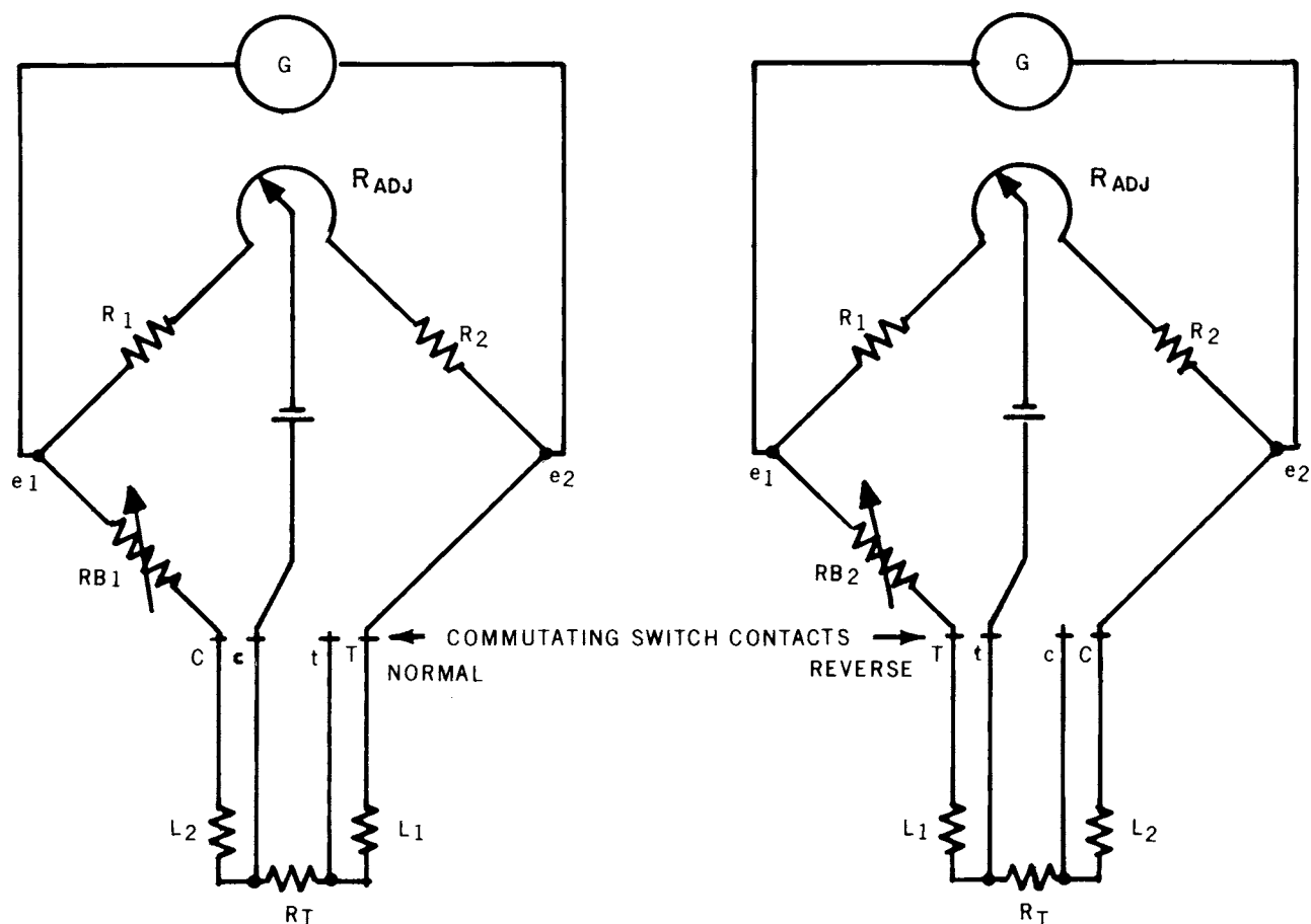
NOTE—Assumes that L_1 = L_2 or that the difference (L_1 - L_2) is constant over the period of measurement. FIG. X1.7 Determination of the Resistance of a Four-Terminal Thermometer Employing a Mueller Bridge
