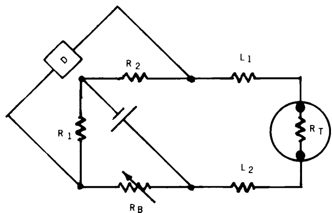
FIG. X1.2 Two-Wire Thermometer Connected to a Simple Bridge
