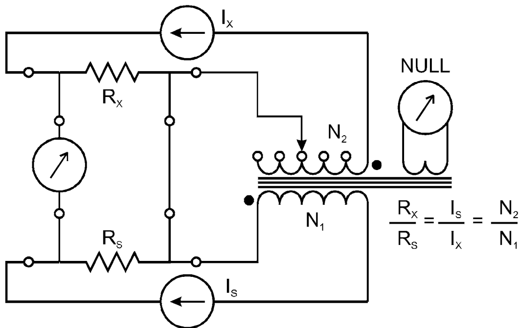
FIG. X2.2 Schematic of DCC Bridge Measurement
