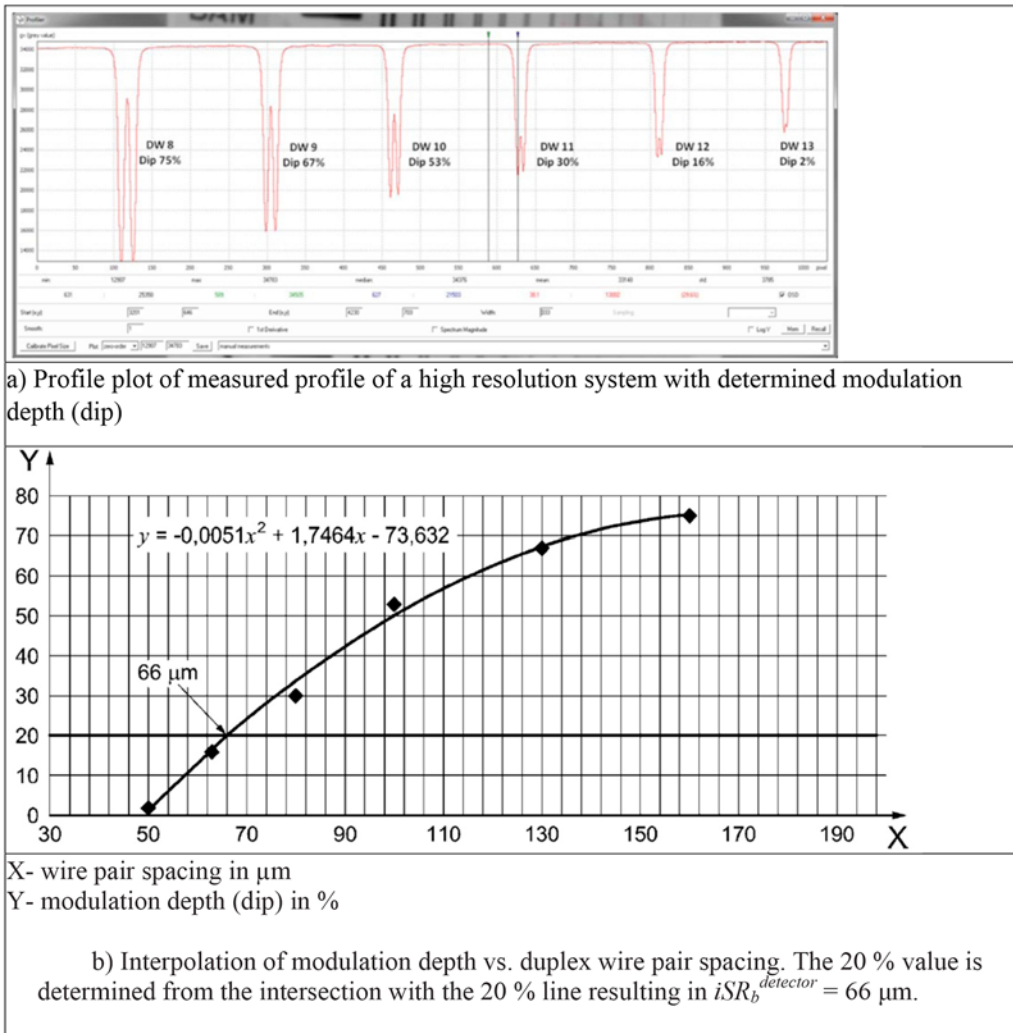
FIG. 4 Wire-Pair Image Analysis for Calculation of interpolated Basic Spatial Resolution of the detector ( iSR_b^{\text{detector}} ).
