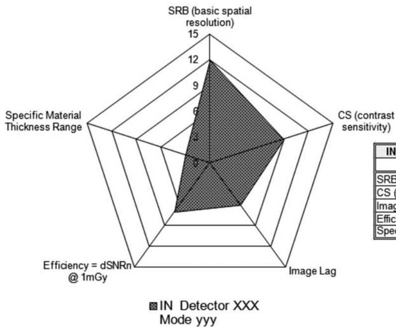
12a. Example DDA potentially suitable for weld inspection.
