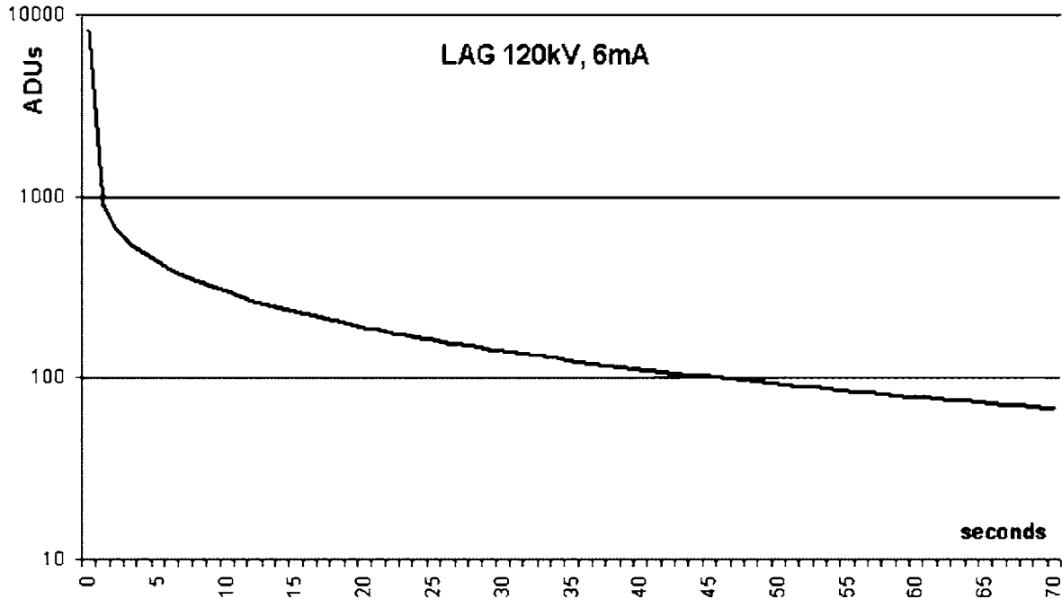
FIG. 9 Result of Image Lag Measurement Sequence
