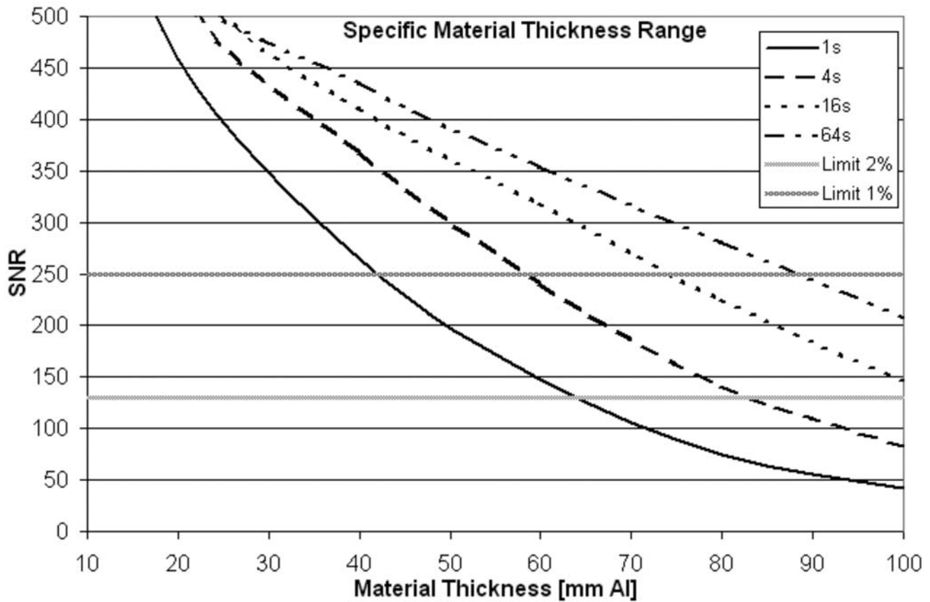
FIG. 8 Specific Material Thickness Range for 2 % Sensitivity at SNR of 130:1 (0 to 84 mm at 4 s exposure time)
