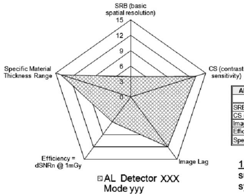
FIG. 12 Net Summary Plots of Some of the Measured Parameters
