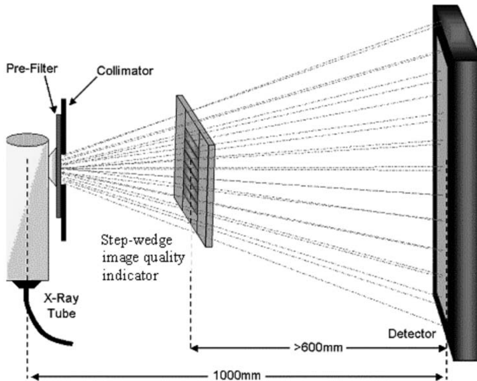
FIG. 4 Scheme of Experimental Arrangement for the Exposure of Step-Wedge Image Quality Indicator
