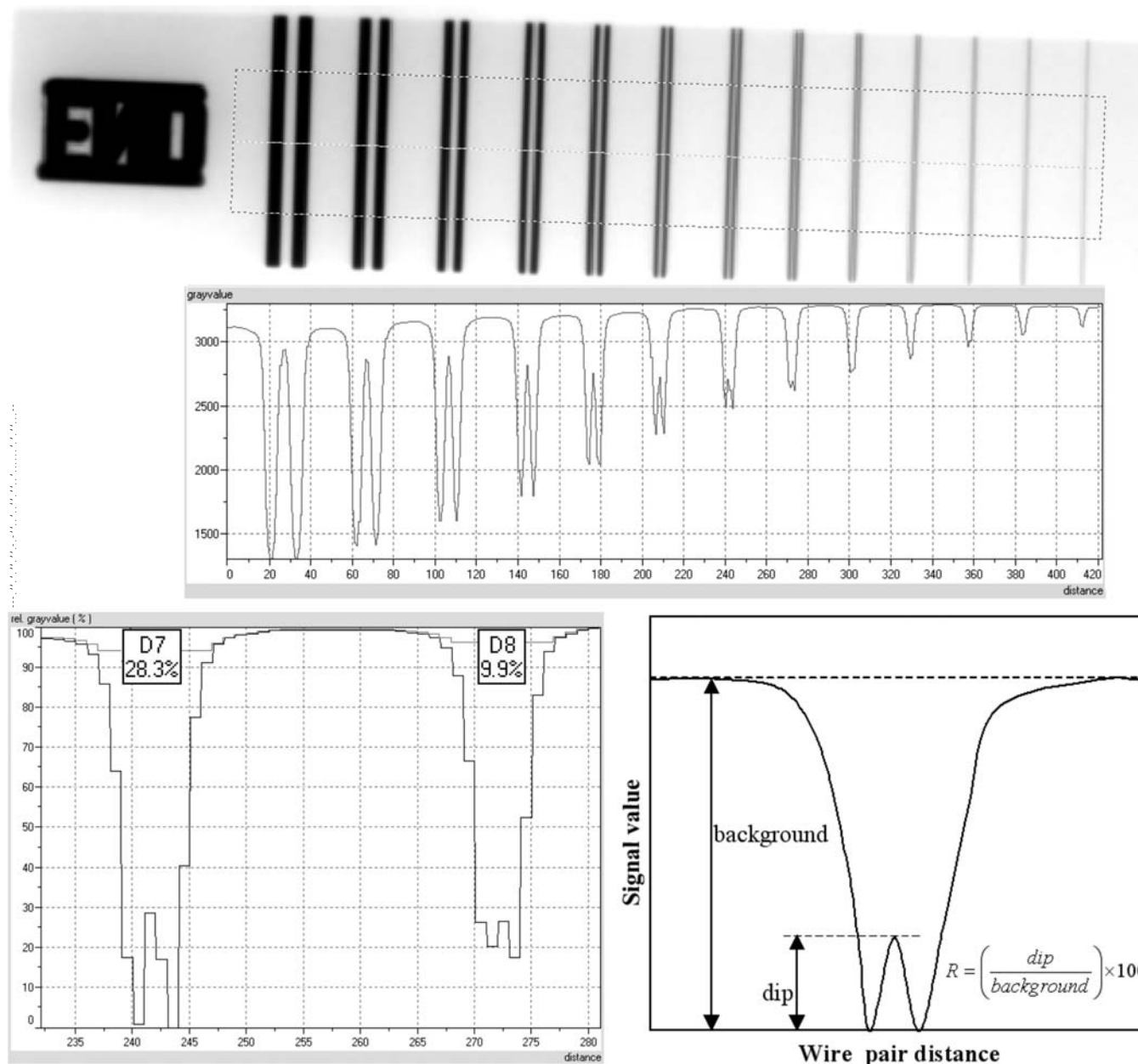
NOTE—Schematic of the measurement is shown at lower right. FIG. 3 Wire-Pair Image Analysis for Calculation of Basic Spatial Resolution
