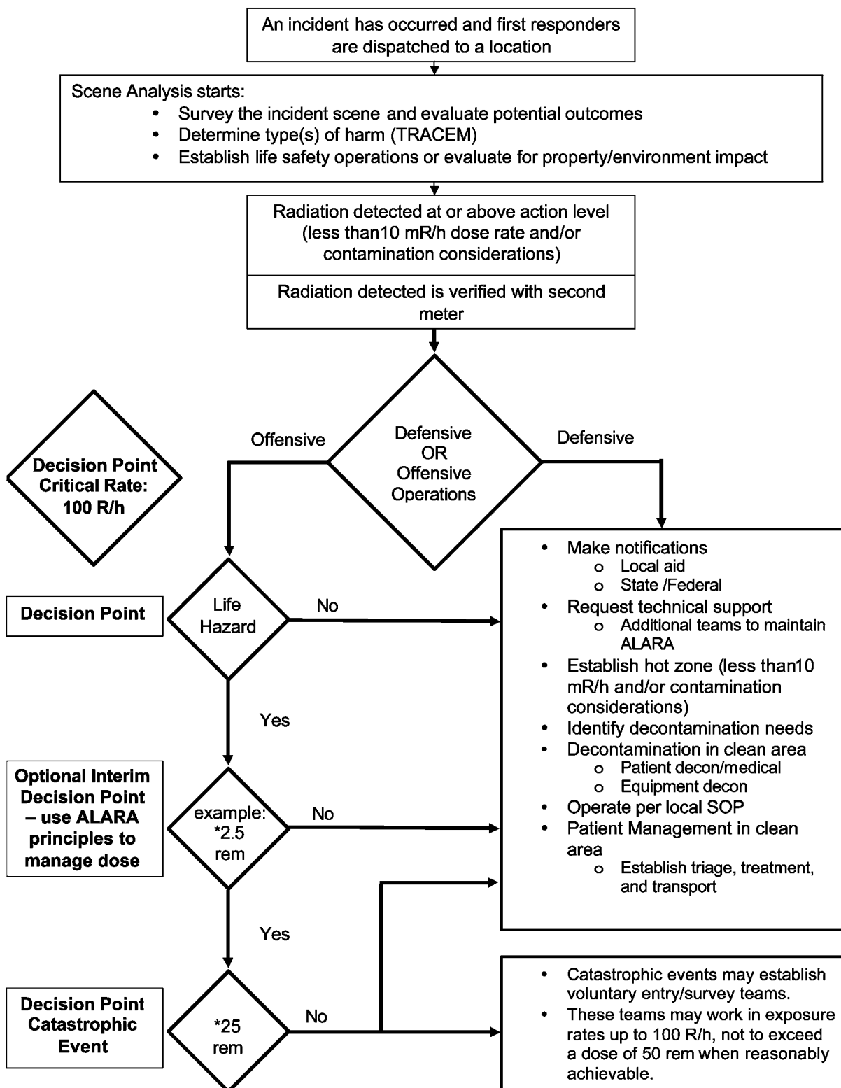
FIG. X8.1 Response Flowchart
