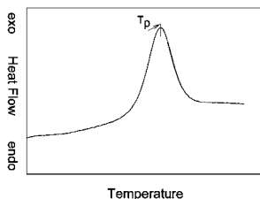
FIG. 1 Example Showing the Temperature of Maximum Heat Flow
