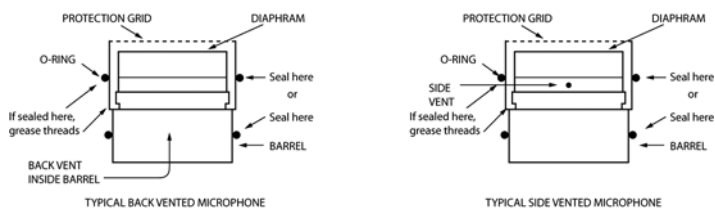
FIG. 2 Microphone Venting and Sealing
