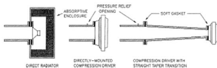
FIG. 1 Sound Source Configuration
