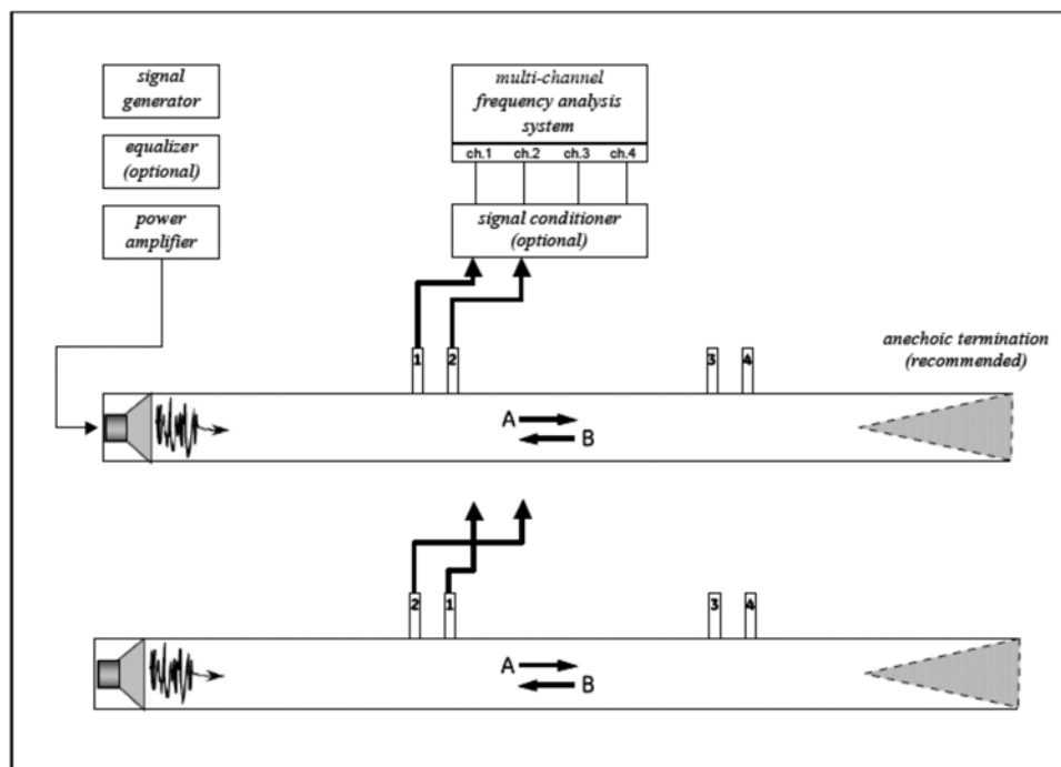
FIG. 5 Apparatus and Instrumentation for Microphone Calibration in the Longitudinal Direction
