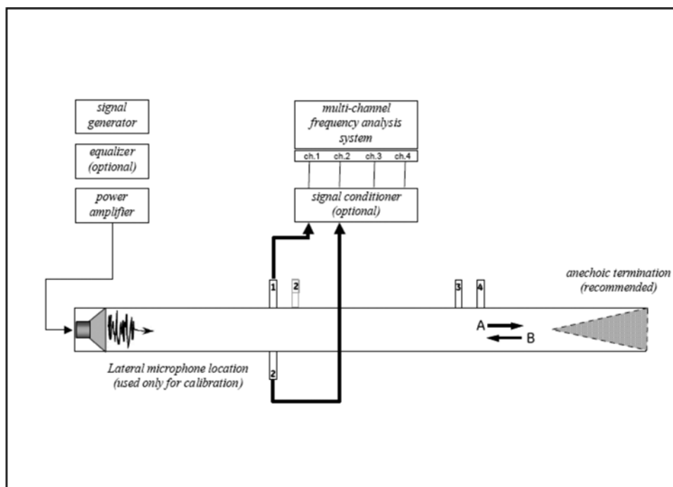
FIG. 6 Apparatus and Instrumentation for Microphone Calibration in the Same Transverse Plane
