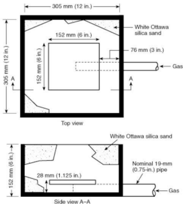
FIG. 2 Schematic Representation of a Gas Burner
