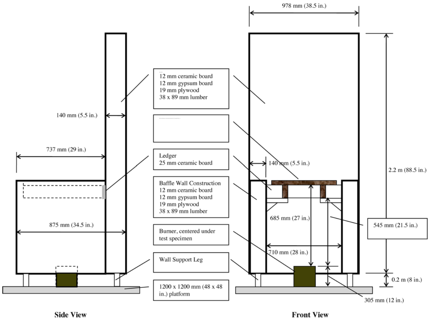
FIG. 1 Schematic Representation of an Under-Deck Test Apparatus
