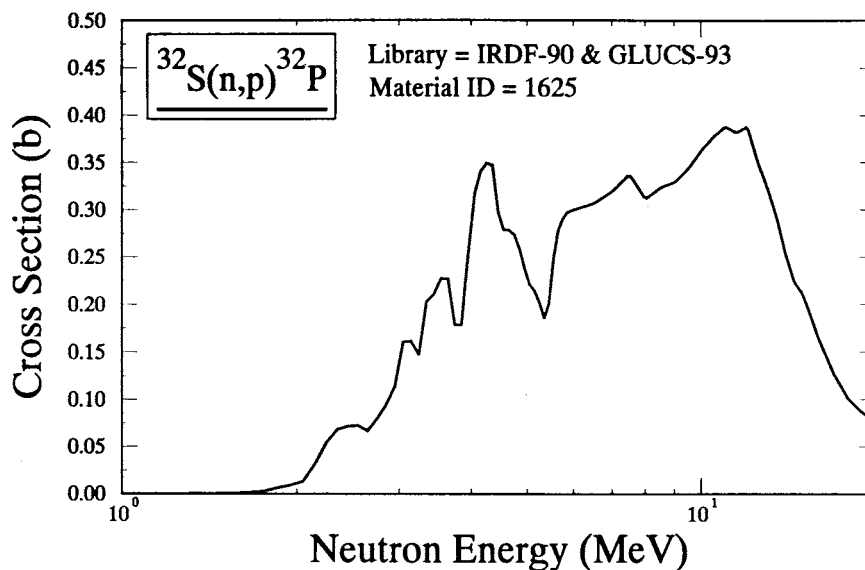
FIG. 1 Cross Section Versus Energy for the ^{32}\text{S}(\text{n},\text{p})^{32}\text{P} Reaction
