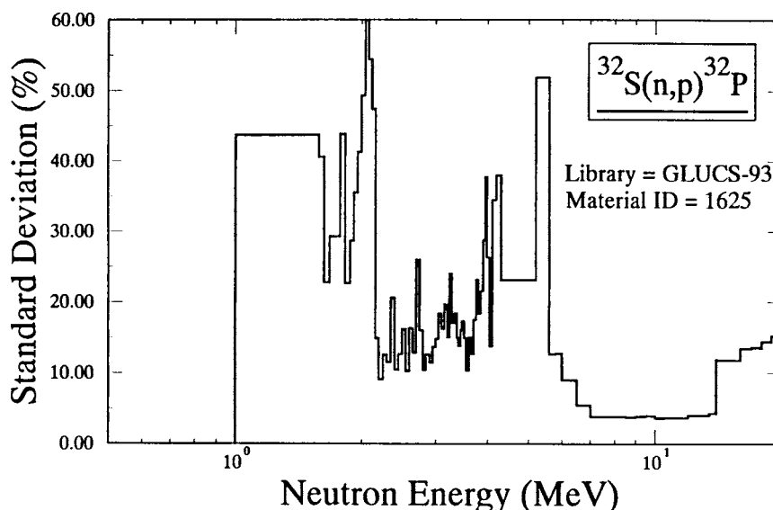
FIG. 2 Energy-dependence of Uncertainty in ^{32}\text{S}(\text{n},\text{p})^{32}\text{P} Cross Section
