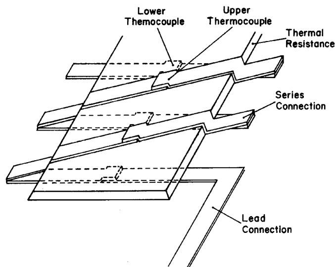
FIG. 3 Isometric View of Thin-Film Gage Pattern
