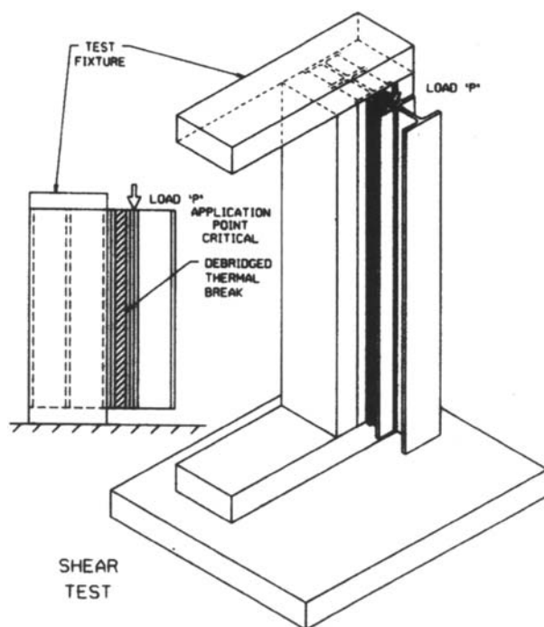
FIG. 2 Shear Test Fixture
