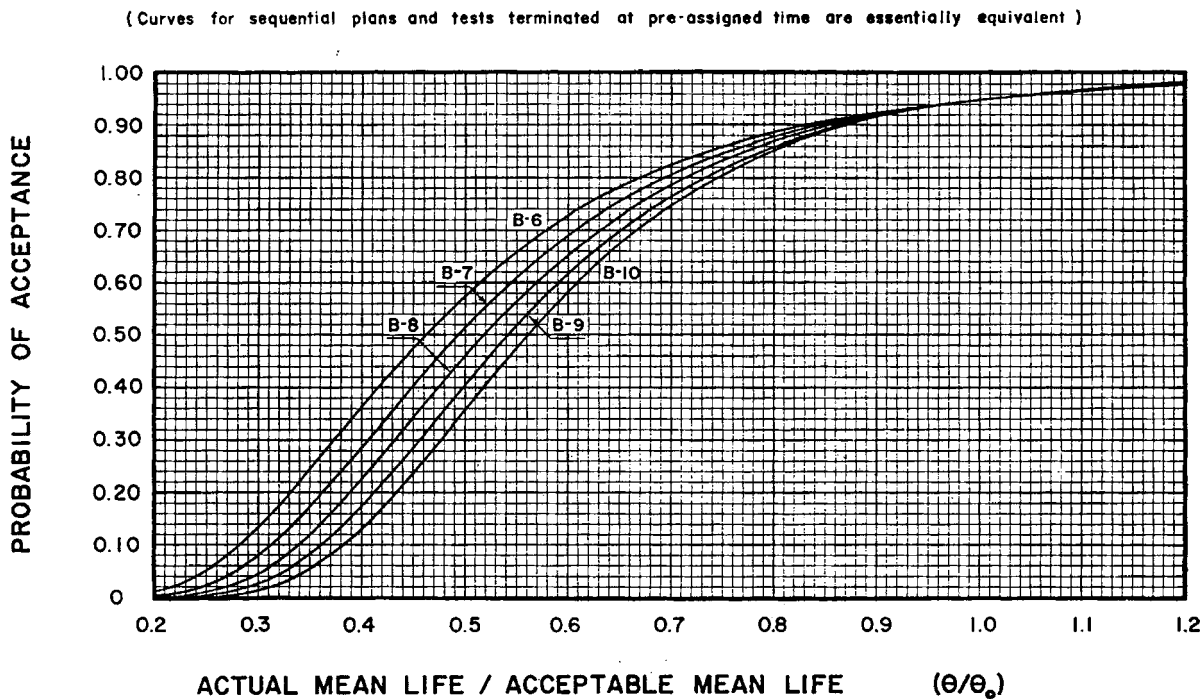
FIG. A1.1 Operating Characteristic Curves for Life Tests Terminated Upon Occurrence of Preassigned Number of Failures (continued)
