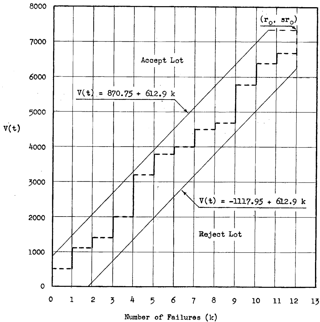
FIG. A1.3 Example of Truncated Sequential Life Test
