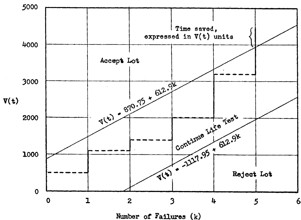
FIG. A1.2 Example of Sequential Life Test
