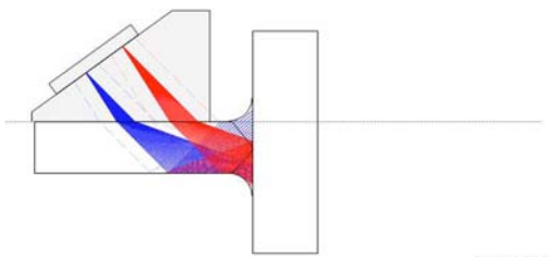
FIG. 4 Corner Welds (Combined S and E Scans)
