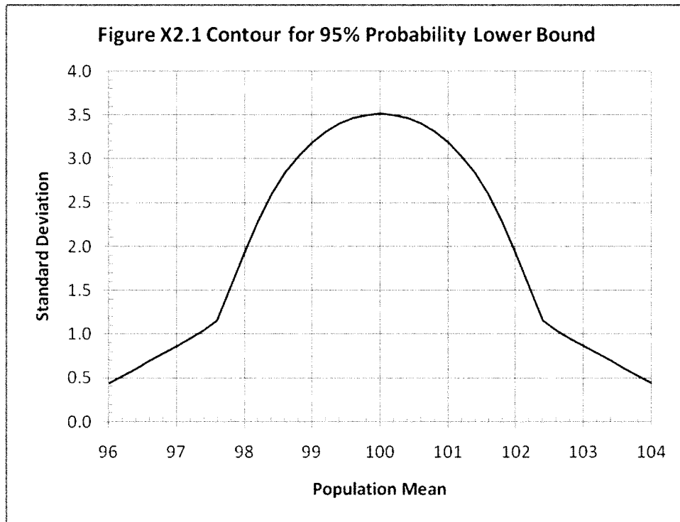
FIG. X2.1 Contour for 95 % Probability Lower Bound
