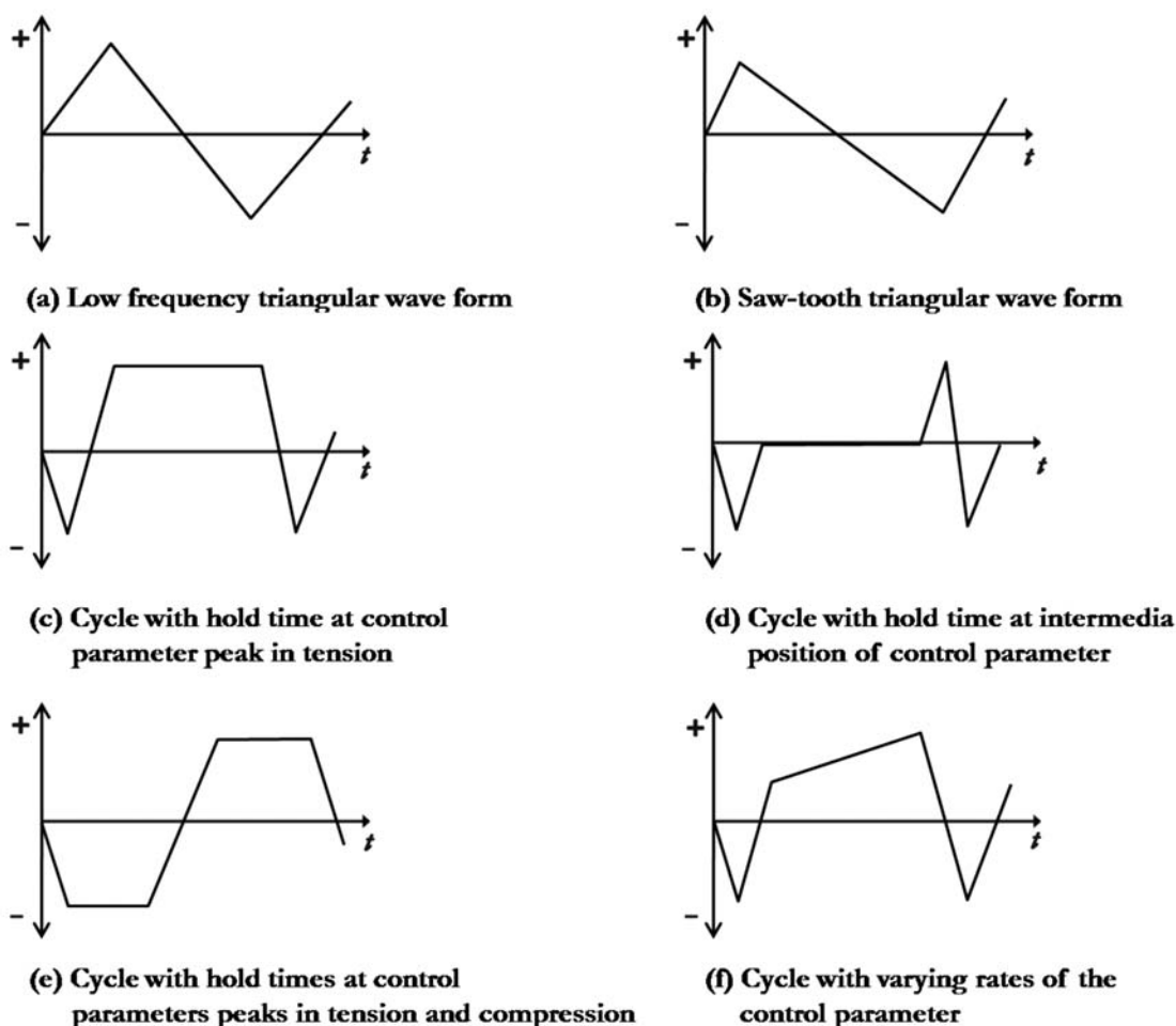
FIG. 3 Example of Creep-Fatigue Cycle Shapes
