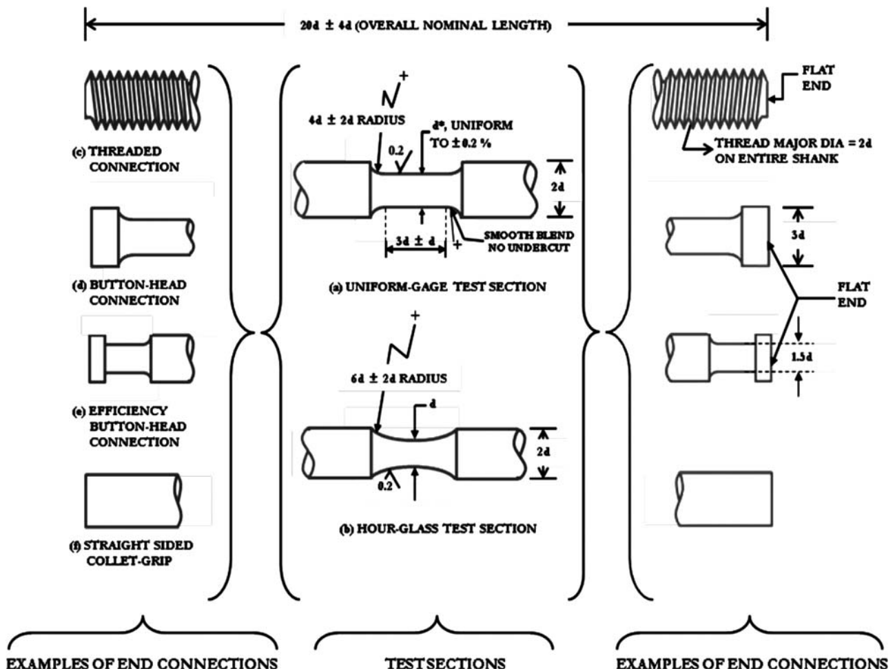
FIG. 5 Test Specimens Configurations
