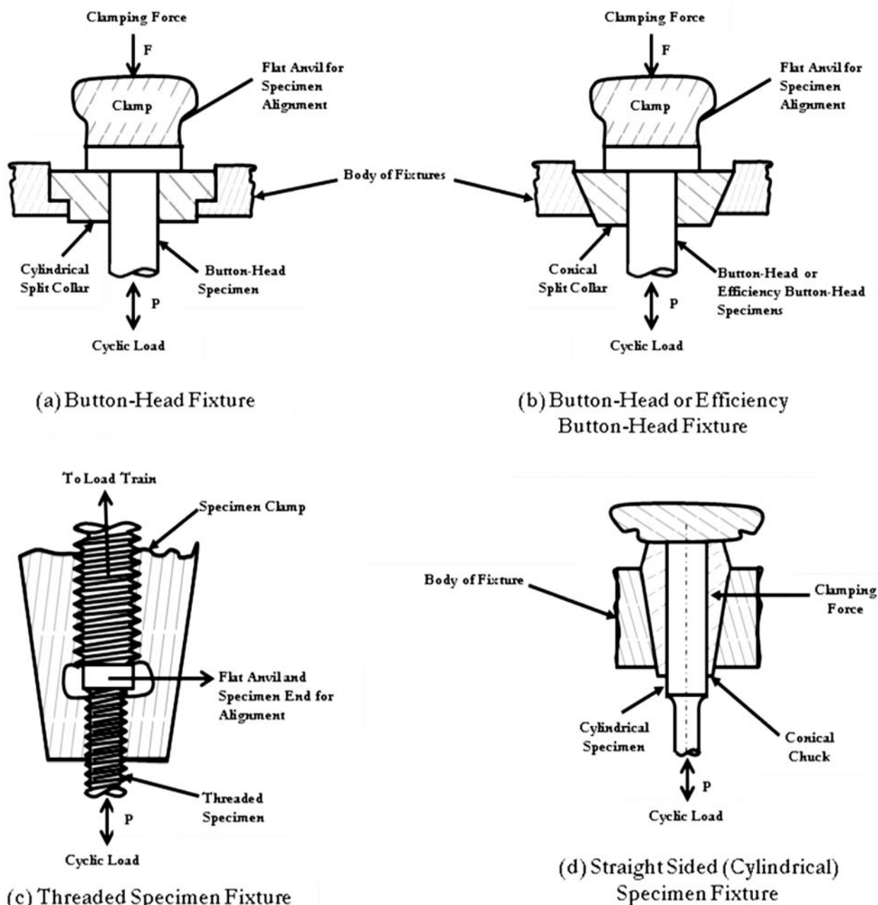
FIG. 6 Schematic Examples of Test Fixtures Suitable for Obtaining Good Alignment and Avoiding Backlash for Various Test Specimen Designs
