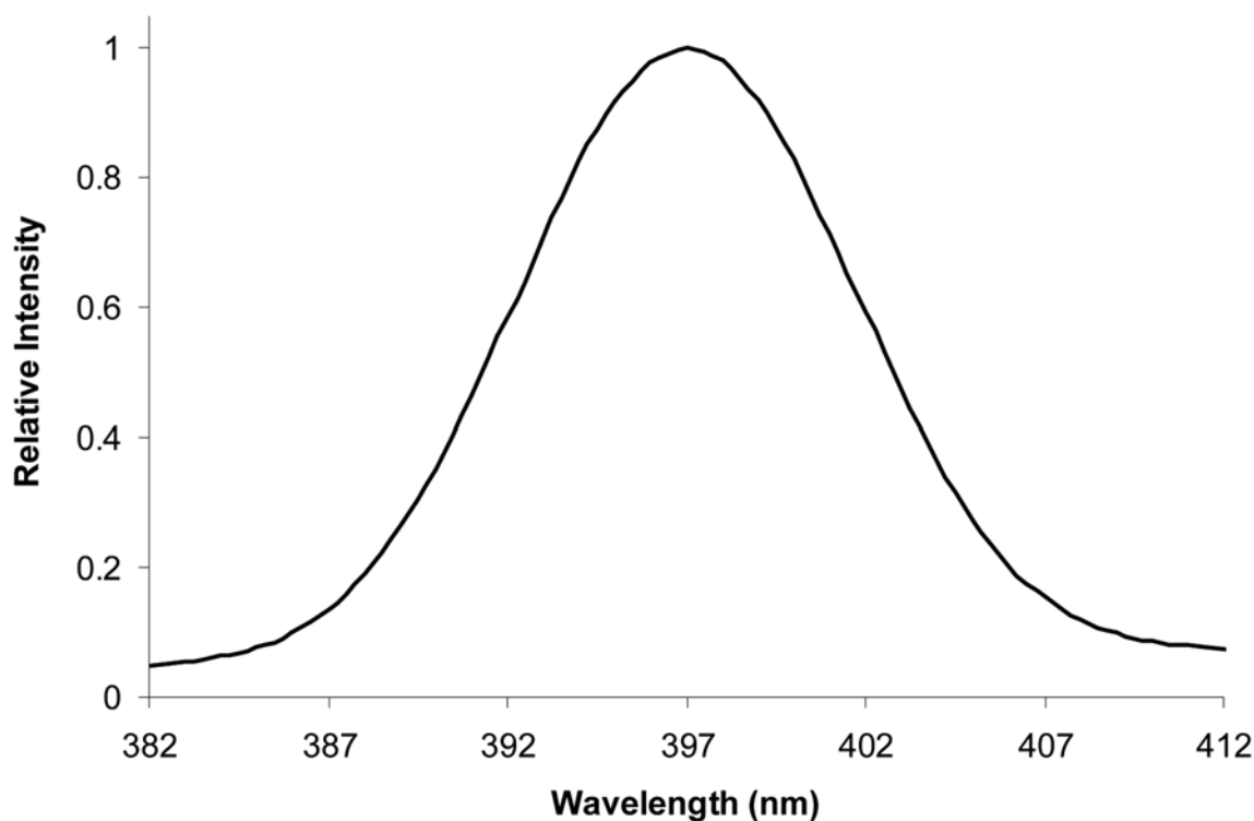
FIG. 8 Water Raman Spectrum with EX Wavelength Set at 350 nm and EX and EM Bandwidths at 5 nm
