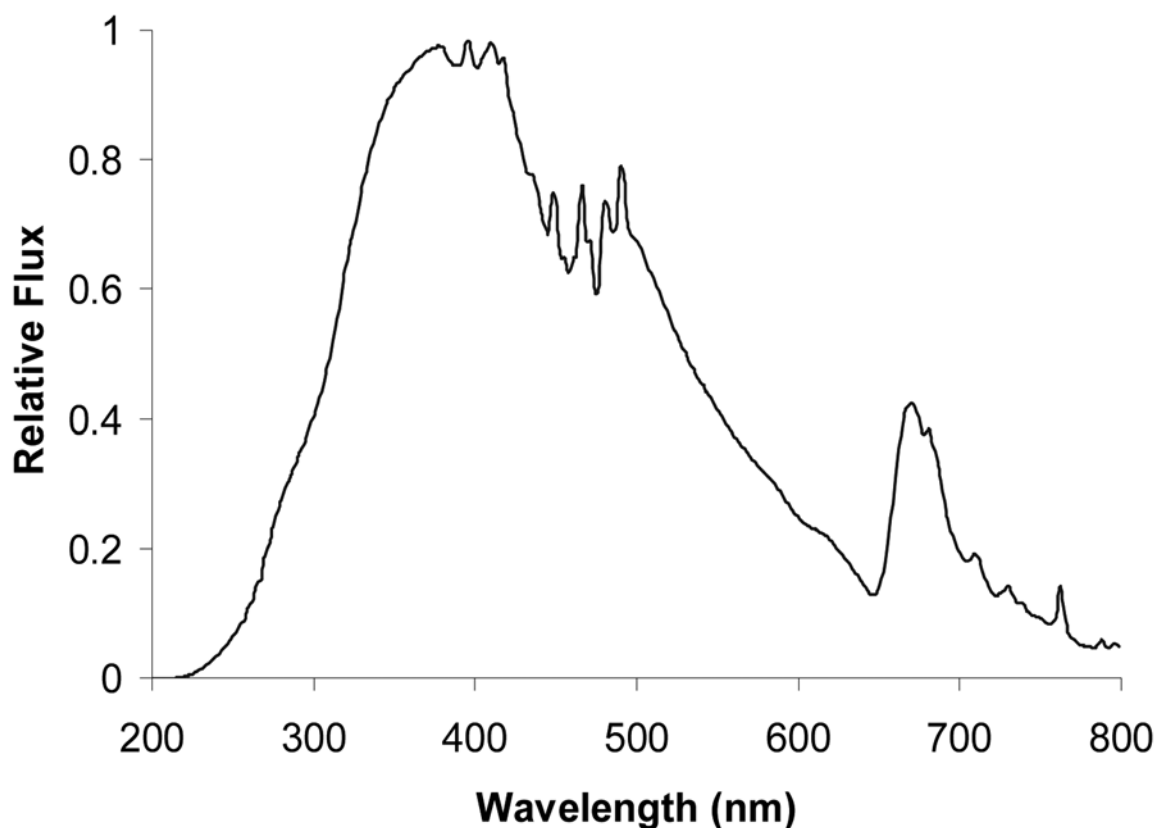
FIG. 10 Example of the Relative Flux of an EX Beam (Xe Lamp-Grating Monochromator Based) (19) for Which a Correction Needs to be Applied to a Measured EX Spectrum to Obtain Its True Spectral Shape (Relative Intensities)
