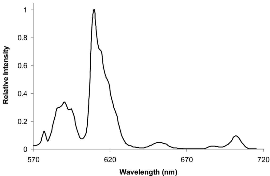
FIG. 3 EM Spectrum of a Eu-Ion-Doped Glass Excited at 392 nm
