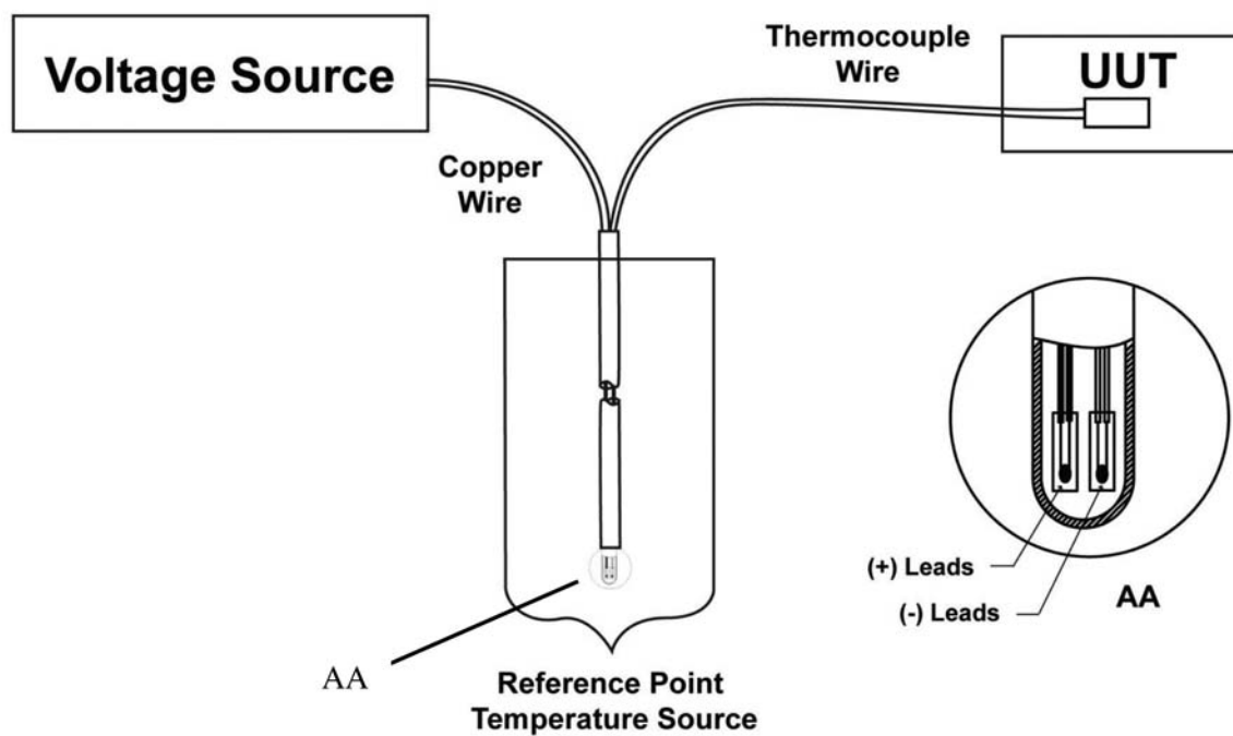
FIG. 5 Schematic Diagram of Usage Mode 2
