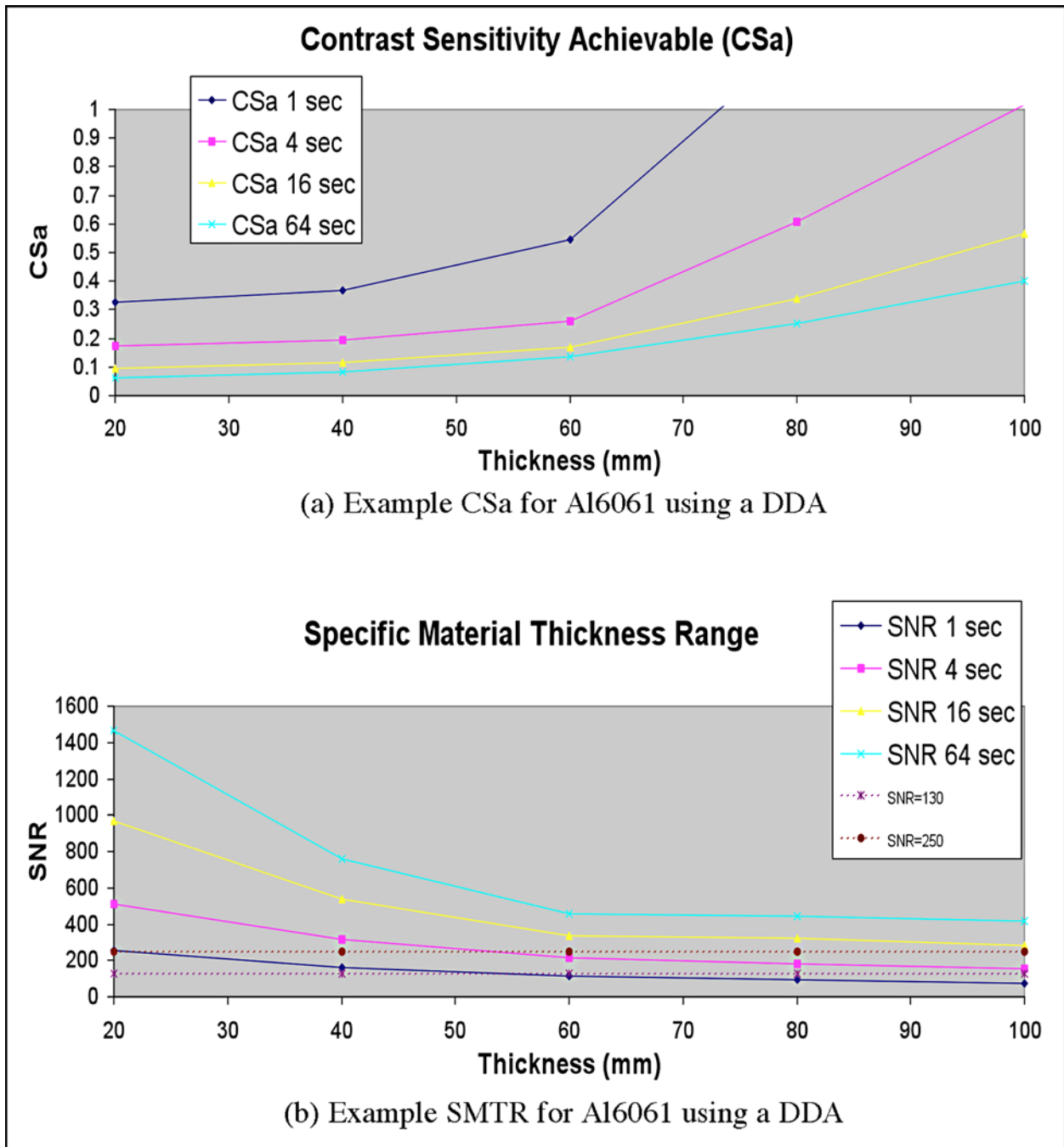
FIG. 8 Example Chart CSa and SMTR for a DDA Using Al6061.
