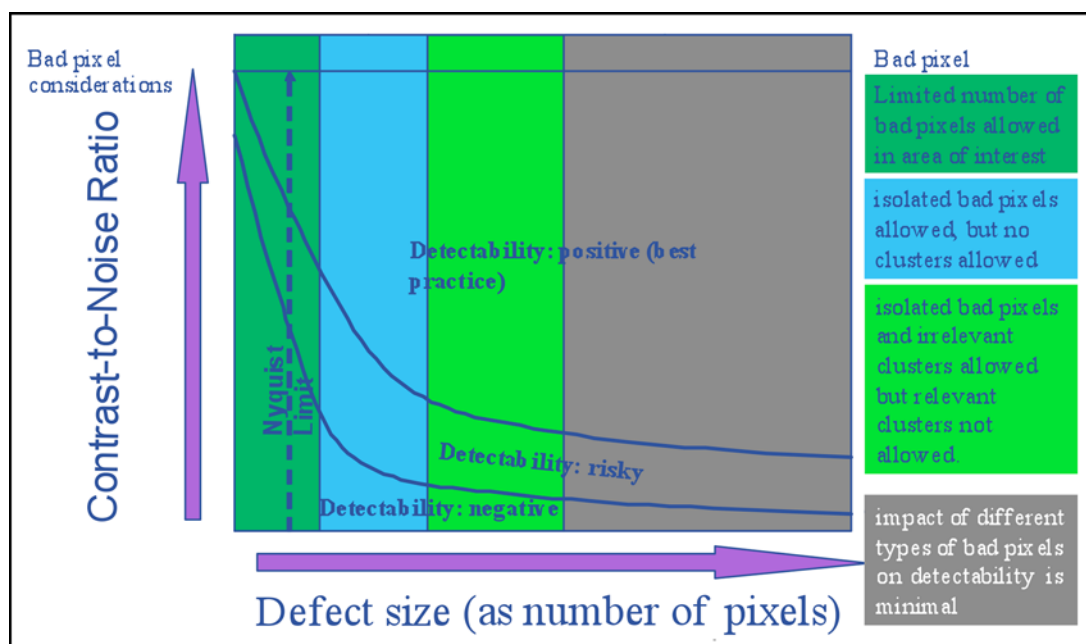
FIG. 11 A Qualitative Guideline for Deciding the CNR Required for a Defect Size and the Bad Pixels Management Rule.
